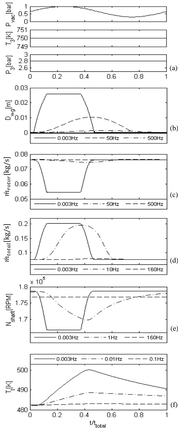
Figure 13: (a) Inlet parameters, (b) waste-gate effective diameter, (c) mass flow through rotor, (d) mass flow through volute, (e) turbo speed and (f) turbine wall temperature for actuator pressure only variation (case 3)
