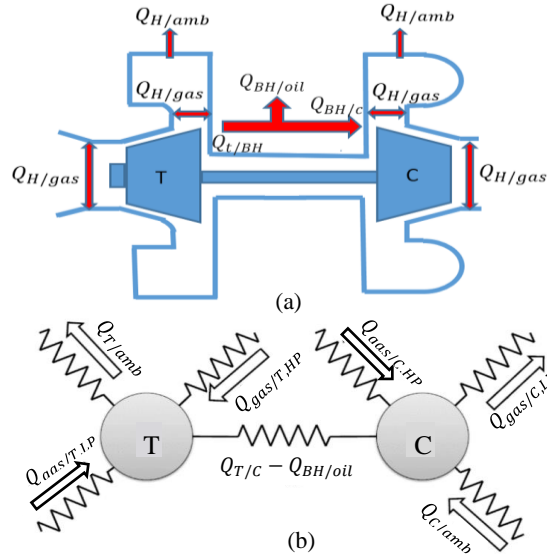
Figure 3: Overview of heat transfer model: (a) schematic of heat transfer process (b) diagram of simplified heat transfer lumped model
