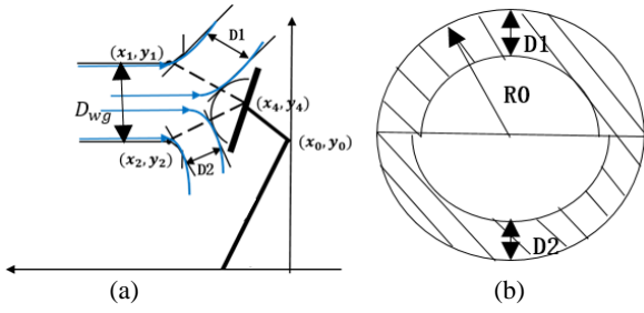
Figure 5: Illustration of waste gate effective area calculation
