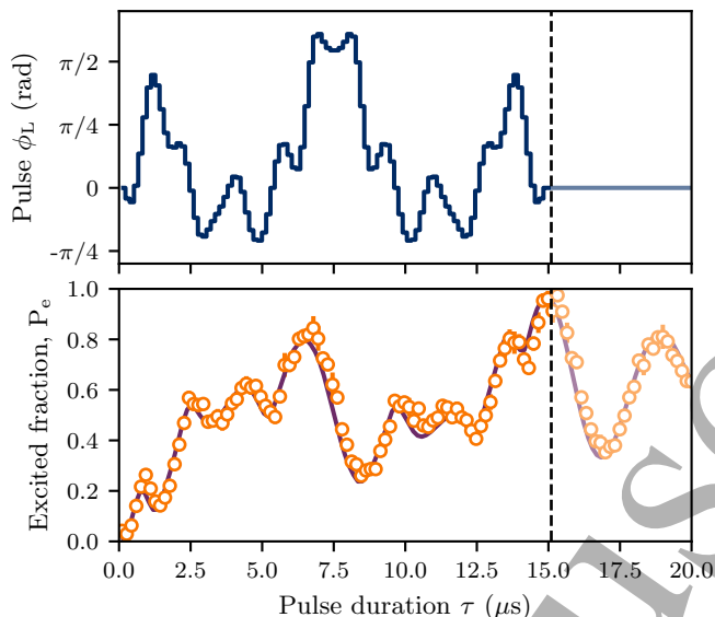
FIG. 6. Above: Optimal state transfer pulse designed using GRAPE to transfer atoms between levels |g\rangle and |e\rangle . Below: Measured fraction (circles) of atoms in the excited state P_e after the Raman light is extinguished at various times during a pulse. The solid line is a theoretical curve produced by the model from [33], in which the two-level Hamiltonian is numerically integrated over the range of detunings and coupling strengths present in a thermal cloud of ^{85}\text{Rb} atoms, and assumes that the light reaches full intensity instantaneously and concurrently with the start of the phase modulation. Excellent agreement is observed for a simulated temperature of 35 \mu\text{K} .
