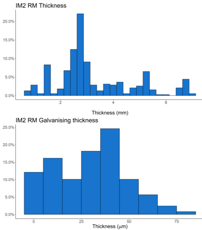
Figure 7 – (Top) Distribution of Rising Main section thicknesses measured in India Mark II hand pumps in Uganda; (Lower) Distribution of Galvanising thickness on Rising Main sections in India Mark II hand pumps.
