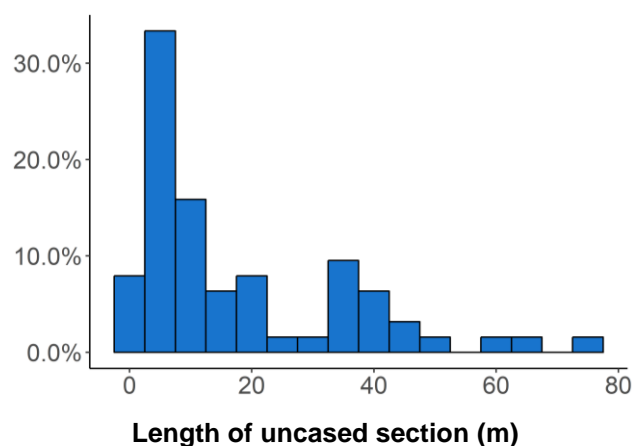
Figure 5 – (Top) the distribution of pump depths in HPBs observed across the four districts in Uganda; (Lower) the typical length of screen or uncased sections in HPB construction.
