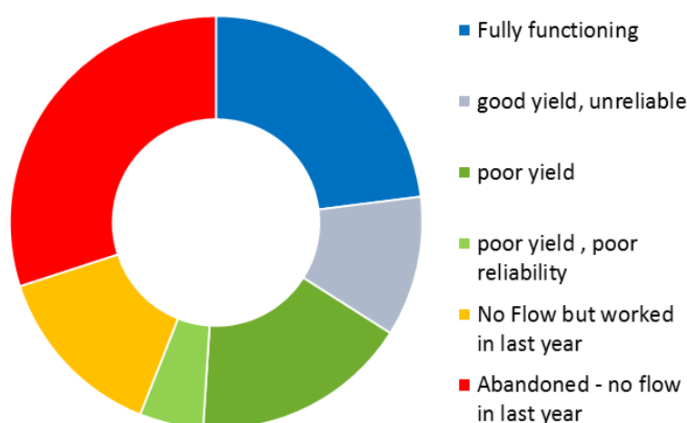
Figure 1 - Functionality performance assessed for boreholes equipped with handpumps within Uganda. The functionality criteria used were: sufficient yield (>10 L/min) on day of survey; and less than 30 days downtime reported for the past year.
