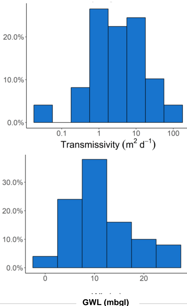
Figure 3 – (Top) Aquifer transmissivity values calculated from pumping test data collected at each of the 50 boreholes; (Bottom) Depth to groundwater (m bgl), measured at each site. The water levels represent a rest water-level following 18 hours of no pumping.
