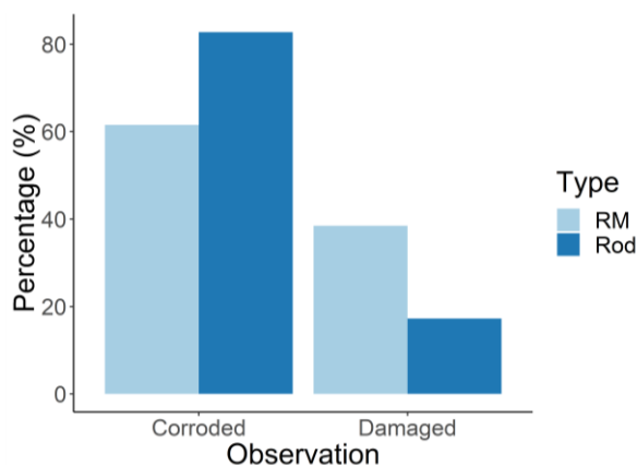
Figure 6 – Percentage of Rising Main (RM) or pump rods which were observed to be damaged or corroded in HPBs in Uganda.
