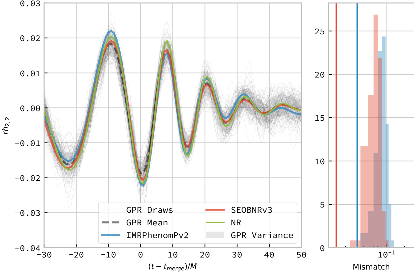
FIG. 7. GPR predictions, compared to NR. One hundred draws from the Gaussian process (left panel) for a non-spinning configuration ( \mathbf{s}_1 = (0, 0, 0) , \mathbf{s}_2 = (0, 0, 0) , \mathbf{q} = 0.625 ), shown as light grey lines compared to the phenomenological approximant models, IMRPhenomPv2 in blue; and SEOBNRv3 in red. The mean draw from the Gaussian process is shown as a grey dashed line, while the associated variance is plotted as a grey-filled region surrounding the mean. The differences between the phenomenological model and the GPR model waveforms are seen to also exist between the phenomenological model waveforms and the NR-derived waveform, plotted here in purple. In the right panel the distribution of mismatches between the samples and both phenomenological waveforms are shown, with the vertical lines representing the mismatch between the mean waveform from the GPR and each phenomenological waveform.
