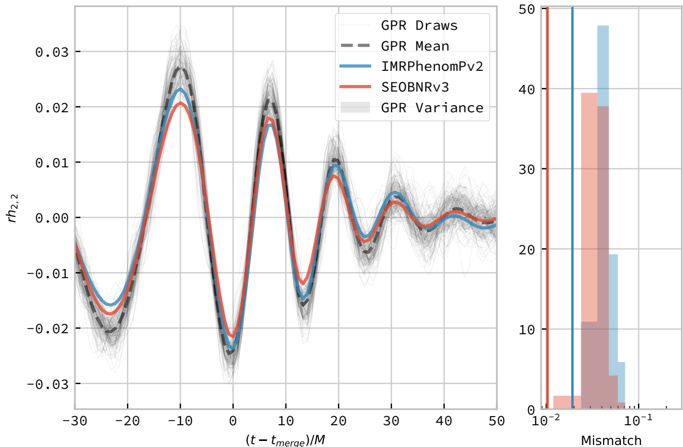
FIG. 4. Non-spinning waveform. One hundred draws from the Gaussian process (left panel) for a non-spinning, equal-mass configuration ( \mathbf{s}_1 = (0, 0, 0) , \mathbf{s}_2 = (0, 0, 0) , \mathbf{q} = 1.0 ), shown as light grey lines compared to two analytical phenomenological approximant models, SEOBNRv3 and IMRPhenomPv2 in red and blue respectively. The mean draw from the Gaussian process is shown as a grey dashed line, while the associated variance is plotted as a grey-filled region surrounding the mean. In the right panel the distribution of mismatches between the samples and both phenomenological waveforms are shown, with the vertical lines representing the mismatch between the mean waveform from the GPR and the phenomenological waveform.
