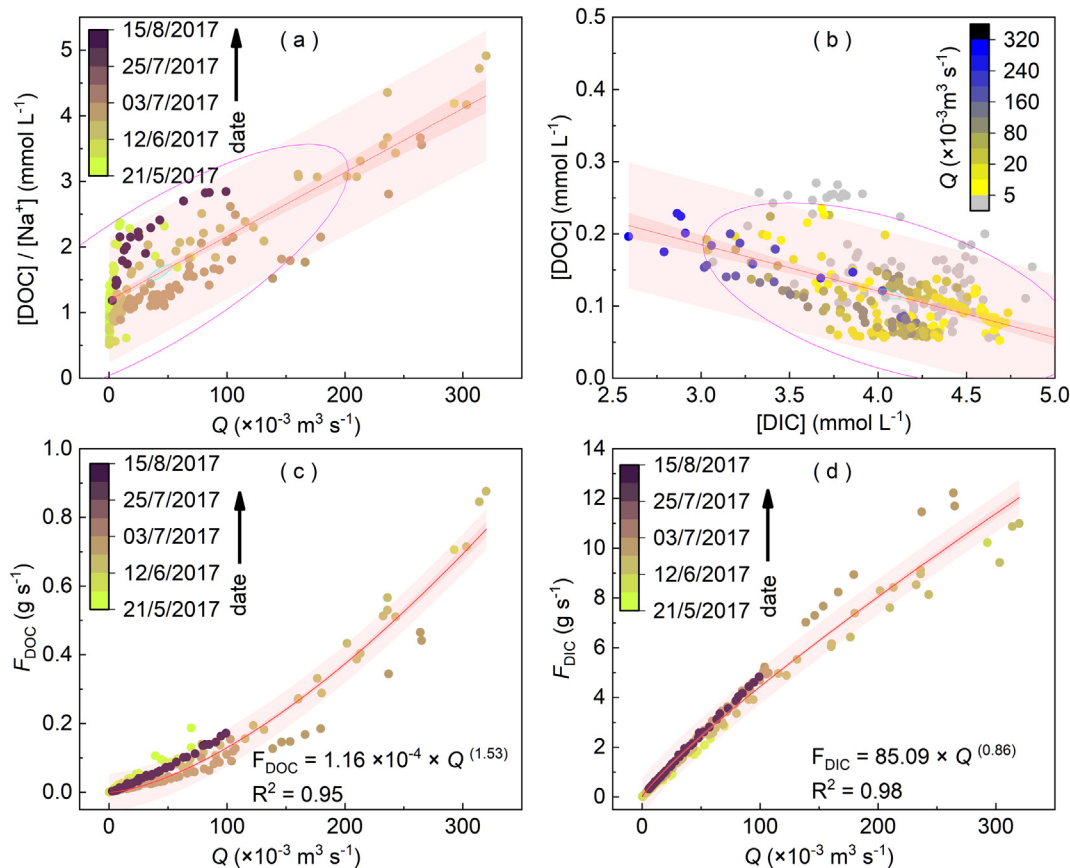
Fig. 9. (a) The relationship between discharge and [\text{DOC}]/[\text{Na}^+] molar ratios. (b) The relationship between DIC and DOC concentrations. (c) Relationships between flux of DOC ( F_{\text{DOC}} ) and discharge. (d) Relationships between flux of DIC ( F_{\text{DIC}} ) and discharge. The little cyan circle and big carmine circle refer to confidence ellipse of mean and prediction, respectively. (For interpretation of the references to color in this figure legend, the reader is referred to the web version of this article.)
