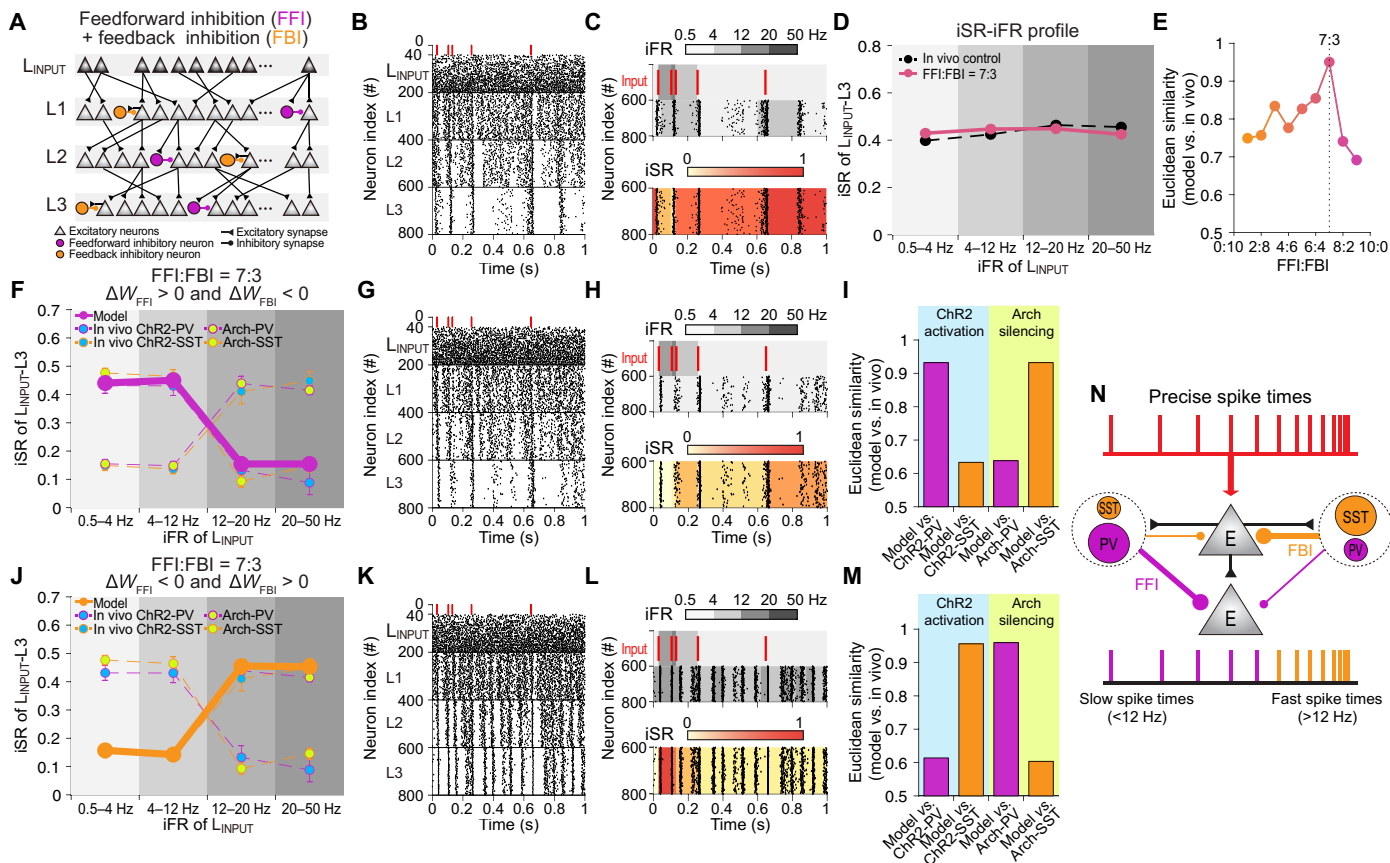
Fig. 4. PV and SST interneurons preferentially recruit feedforward and feedback inhibition for frequency-selective gating of spike-timing synchronization. (A) Schematic of a three-layer network model consisting of 200 single-compartment Hodgkin-Huxley excitatory neuron models (triangles) and 50 inhibitory interneuron models (circles) that provide feedforward inhibition (FFI; magenta) and feedback inhibition (FBI; orange) at 7:3 ratio. (B) Spike raster plot of the model in response to spike-timing sequence recorded in granular layer in S1 in vivo (red). Dots indicate spikes. A subset of neurons (40 neurons) in the input layer ( L_{INPUT} ) received the input (red dots), while the rest spiked spontaneously (black dots), reflecting sparseness. (C) Representatives of iFR (four bins: 0.5 to 4, 4 to 12, 12 to 20, and 20 to 50 Hz, gray color scale; top) and iSR (maximum 1, red color scale; bottom) of neurons in L_{INPUT} -L3 pair in each model. Red lines in L_{INPUT} are the input spike-timing sequences. Black dots are spikes in L3. (D) iSR-iFR profile of network model with FFI:FBI ratio at 7:3 (pink). In vivo-recorded iSR-iFR profile in the control condition (black filled circles, black dashed line) are plotted together for comparison. (E) Euclidean similarity of iSR-iFR profiles between in vivo data in control condition and simulation of the network model with different ratio of FFI:FBI showing 7:3 as the optimal ratio for the synchronization of spike times. Different ratios of FFI:FBI color-coded as different shades of magenta to orange. (F) iSR-iFR profile in response to increase in synaptic weights of FFI ( \Delta W_{FFI} > 0 ) complemented by decrease in synaptic weights of FBI ( \Delta W_{FBI} < 0 ) in the network model to balance inhibition (filled magenta circle). ChR2-PV activation (blue filled circles, magenta dashed line), ChR2-SST activation (blue filled circles, orange dashed line), Arch-PV silencing (green filled circles, magenta dashed line), and Arch-SST silencing (green filled circles, orange dashed line) are plotted together for comparison. In vivo data represent means \pm SEM. (G and H) Same as (B) and (C) but in a network model with \Delta W_{FFI} > 0 and \Delta W_{FBI} < 0 in the model. (I) Four-dimensional Euclidean similarity of iSR-iFR profiles between in silico model in (F) and in vivo data in each condition. Magenta bar, optogenetic manipulation of PV interneuron in vivo; orange bar, optogenetic manipulation of SST interneuron in vivo. Blue and green shades indicate ChR2 activation with blue light and Arch silencing with green light in each interneuron subtypes, respectively. (J to M) Same as (F) to (I) but with \Delta W_{FBI} > 0 complemented by \Delta W_{FFI} < 0 in the network model to balance inhibition. The corresponding iSR-iFR profile is shown in filled orange circles in (J). (N) Cartoon summarizing the frequency-selective gating of spike-timing synchronization by PV and SST interneurons through preferential activation of FFI and FBI.
