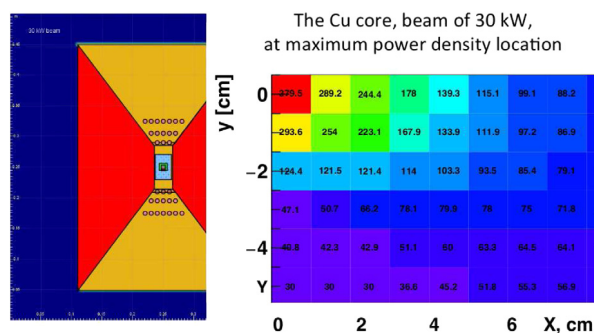
Fig. 7. Left panel: the cross section of the absorber with the water cooling channels (the copper is shown in light blue and the W-Cu(20%) is shown in gold). Right panel: the temperature map for 1 cm by 1 cm elements at the longitudinal coordinate of the power deposition maximum. (For interpretation of the references to color in this figure legend, the reader is referred to the web version of this article.)
