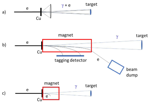
Fig. 1. Different schemes to produce high-energy photon beams. Scheme (a) is the traditional bremsstrahlung technique where a copper radiator is placed in an electron beam resulting in a mixed photon and electron beam. In scheme (b) a deflection magnet and beam dump are used to peel off the electrons and produce a photon-only beam. Scheme (c) is the new CPS technique, with a compact hermetic magnet-electron dump and a narrow pure photon beam.
