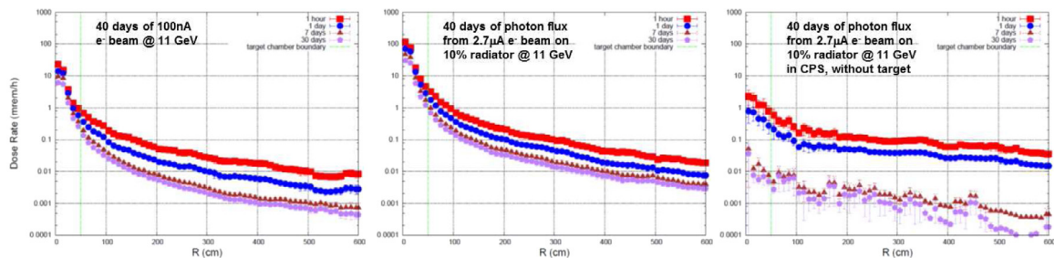
Fig. 18. Activation dose rate at the target for different configurations. Distance R is radial distance from the target center, with the radius of the scattering chamber boundary located at 50 cm.
