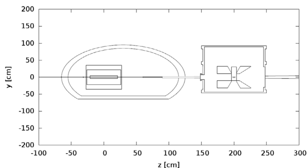
Fig. 15. An alternative shielding design used in FLUKA radiation calculations with reduced W-powder overall, on the bottom-side and with rounded corners.
