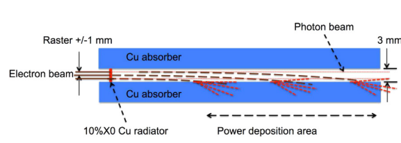
Fig. 4. The scheme of beam deflection in the magnetic field to the absorber/dump.
