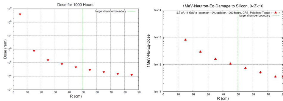
Fig. 20. The prompt radiation dose (left) and the resulting 1 MeV neutron equivalent damage to silicon (right) in the target area, assuming the conditions described above. The polarized target system is centered at R = 0 , the nominal target chamber radius is 50 cm and the target coils are at about 20 cm from the beam line. The dose at the target coils is 5 \times 10^5 rem and the 1 MeV neutron equivalent damage is 5 \times 10^{12} neutrons/cm 2 .
