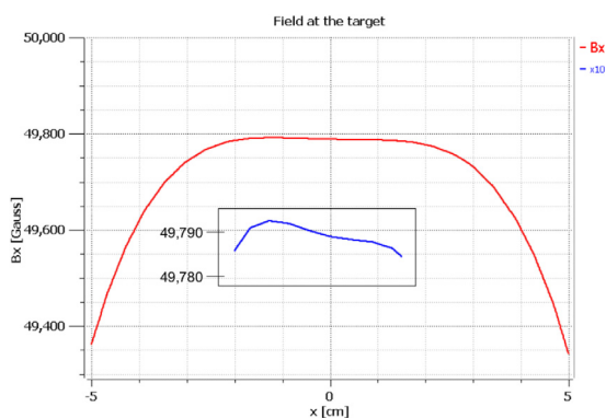
Fig. 10. The field at the target center. The insert shows the field zoomed by a factor of 10.
