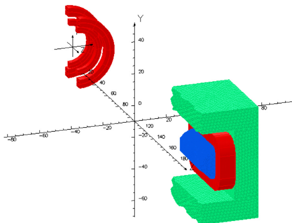
Fig. 9. The TOSCA model used in the field and force calculations for longitudinal orientation of the coils/target polarization.
