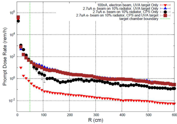
Fig. 17. Prompt dose at the target for different configurations. Distance R is radial distance from the target center, with the radius of the scattering chamber boundary located at 50 cm.
