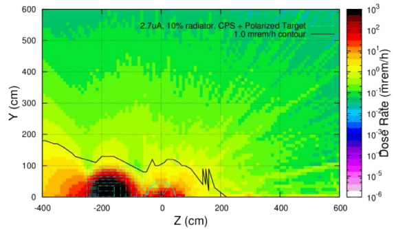
Fig. 19. Activation radiation dose rate one hour after a 1000-h experiment as a function of position in the experimental hall for the case of a 2.7 \mu\text{A} electron beam hitting a 10% copper radiator inside the CPS, with the target geometry included. The 1 mrem/h contour is indicated.
