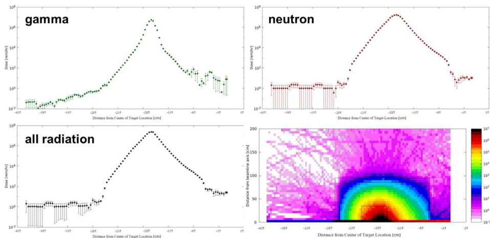
Fig. 13. Prompt radiation dose rate as a function of position in the experimental hall for the case of a 2.7 \mu\text{A} electron beam hitting a 10% copper radiator inside the CPS. One-dimensional plots are shown for the dose from photons only (top left), from neutrons only (top right) and from all particle types (bottom left). Also shown is a two-dimensional plot of prompt dose rate (bottom right), which shows the effectiveness of the CPS shielding concept.
