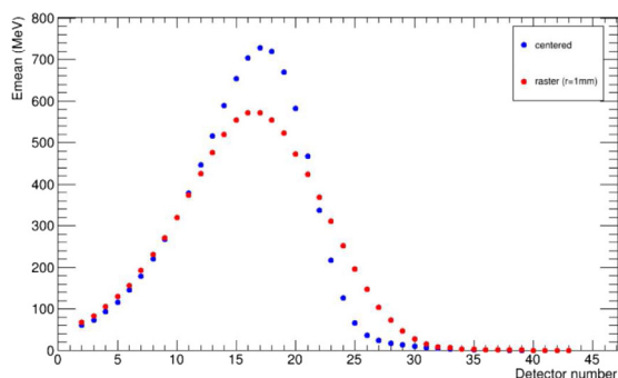
Fig. 6. Longitudinal profile of the energy distribution (integrated for one cm copper slab) for a 11 GeV incident electron beam. The maximum power density occurs at a distance of 18 cm from the radiator. The blue dots show the energy deposition for the electron beam centered in a 3 mm by 3 mm channel, while the red dots show the same for the beam rastered with a radius of 1 mm. (For interpretation of the references to color in this figure legend, the reader is referred to the web version of this article.)
