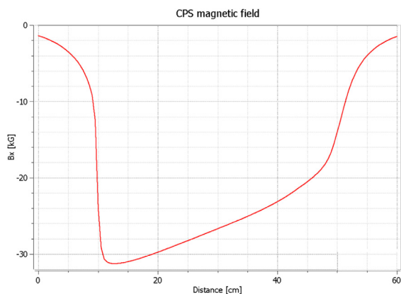
Fig. 5. Magnetic field ( B_x ) profile along the beam direction, as a function of distance from the radiator position.
