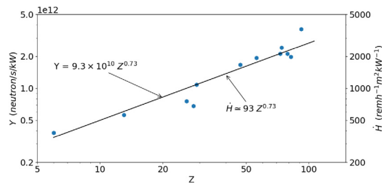
Fig. 8. The neutron yield and dose rate for a 500 MeV incident electron beam as a function of atomic number (based on an original figure from SLAC [45]).
