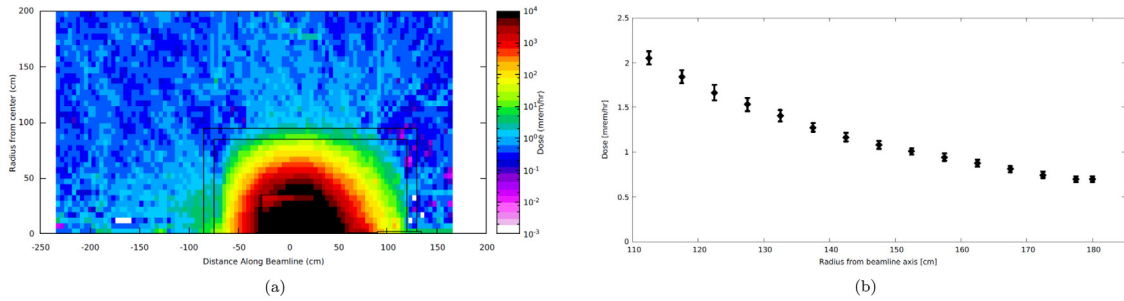
Fig. 16. Activation radiation dose rate one hour after a 1000-h experiment as a function of position in the experimental hall for the case of a 2.7 \mu\text{A} electron beam hitting a 10% copper radiator inside the CPS.
