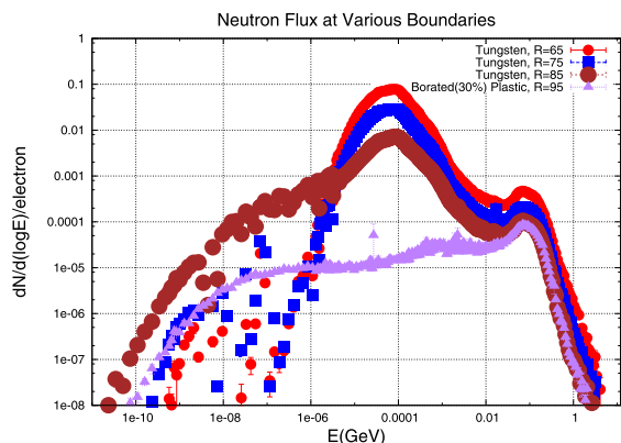
Fig. 14. Neutron flux escaping the CPS for different shielding configurations, including the use of borated plastic.
