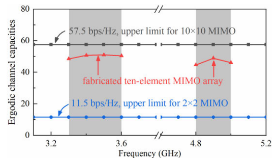
FIGURE 16. Calculated ergodic channel capacities of the fabricated antenna array.
