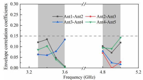
FIGURE 15. Calculated ECCs of the fabricated antenna array.
