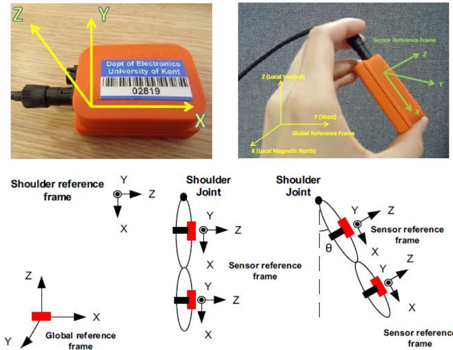
Figure 1 Reference frames for the XSens MTx inertial sensor system.
