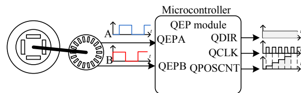
Fig. 2. Interface of the microcontroller with an incremental sensor.
