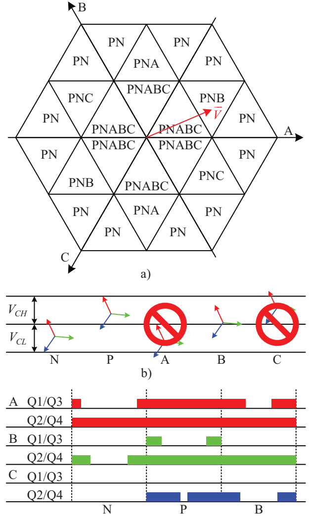
Fig. 2. Three-level inverter possible PWM patterns (a); examples of vector implementations (b); PWM patterns for each case (c).
