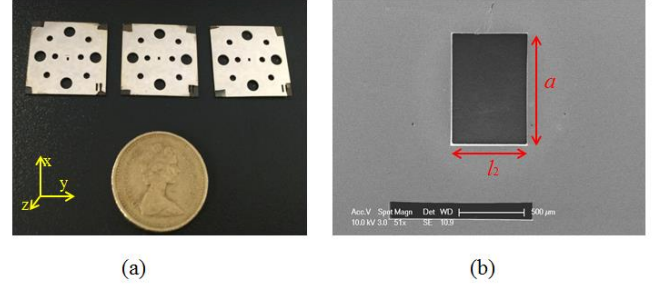
Fig. 6. (a) Photograph of the 3 silver-coated SU-8 layers, 20 × 20 mm for each layer with a thickness of 0.432 mm. (b) Scanning electron microscope image of the cavity structure for the second SU-8 layer.
