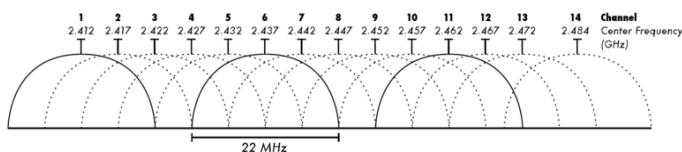
Figure 2: Wifi Channel Allocation (Lammle, T., (2007))
