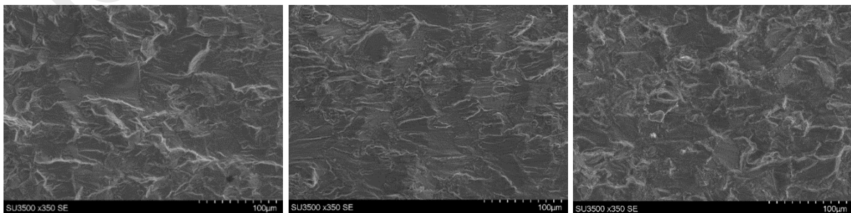
Figure 10: OP TMF CG RR1000 fracture surfaces at 350x magnification under \Delta T=400-750^\circ\text{C} no dwell (left), \Delta T=400-775^\circ\text{C} no dwell (centre) and \Delta T=350-750^\circ\text{C} 120s dwell at peak temperature (right).
