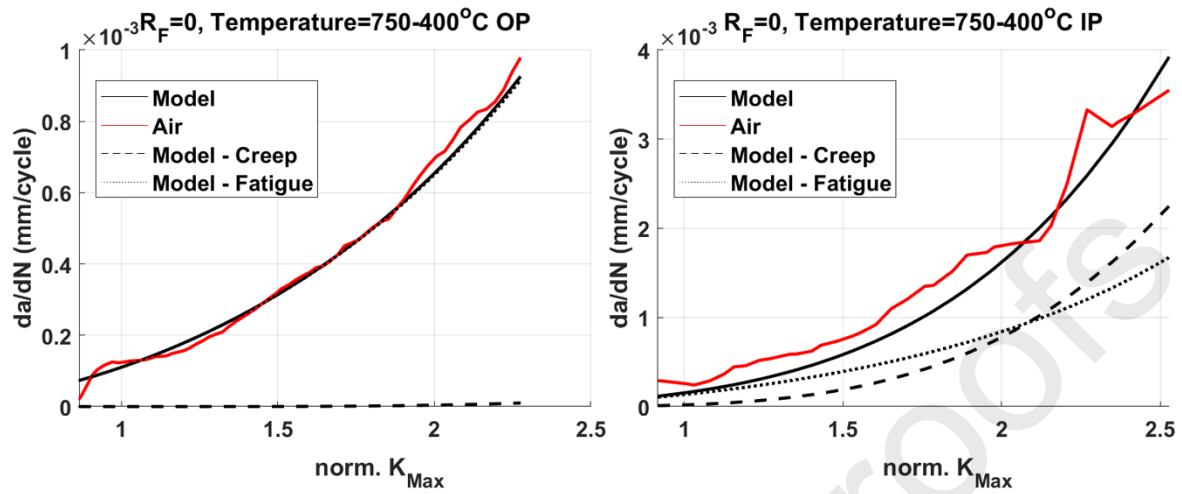
Figure 14: Crack growth prediction for OP (left) and IP (right) test under thermo-mechanical fatigue loading.
