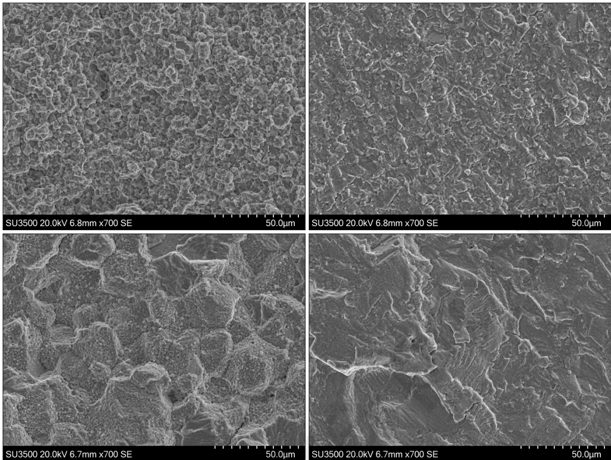
Figure 7: Fracture surfaces of IP and OP, TMF experiments displayed in Figure 5a at 350-750°C on FG and CG variants of RR1000 at x700 magnification. IP FG (top left), OP FG (top right), IP CG (bottom left) and OP CG (bottom right).
