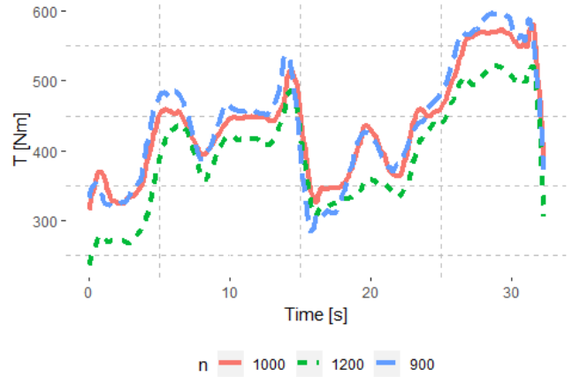
Figure 3. Load cycle in Nm for n=900 (blue), n=1000 (red) and n=1200 (green) rpm in validation tests
