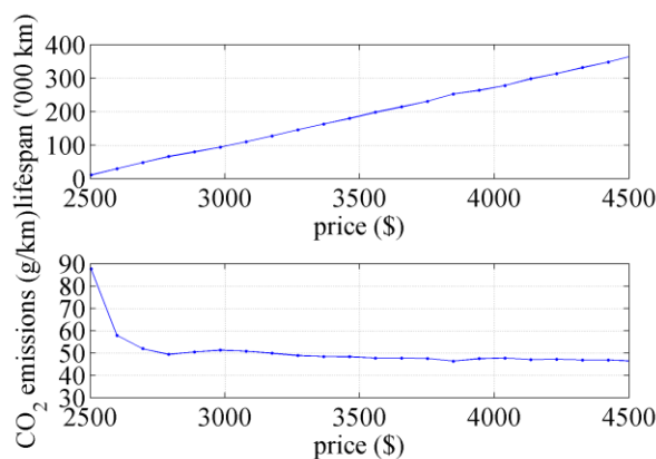
Figure 4. Battery trade-offs
