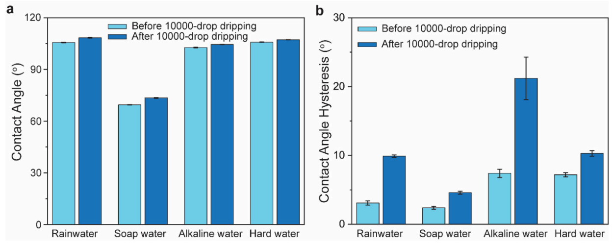
Supplementary Figure 3. Plots showing (a) contact angle and (b) contact angle hysteresis of various liquids on LESS-coated surfaces before and after 10000-droplet dripping. All error bars represent standard deviations of three independent measurements.
