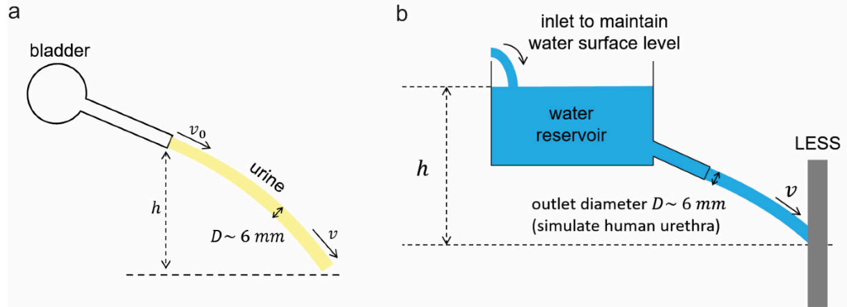
Supplementary Figure 14. Schematic showing (a) a physical model and (b) a flow setup to emulate the process of human urination.
