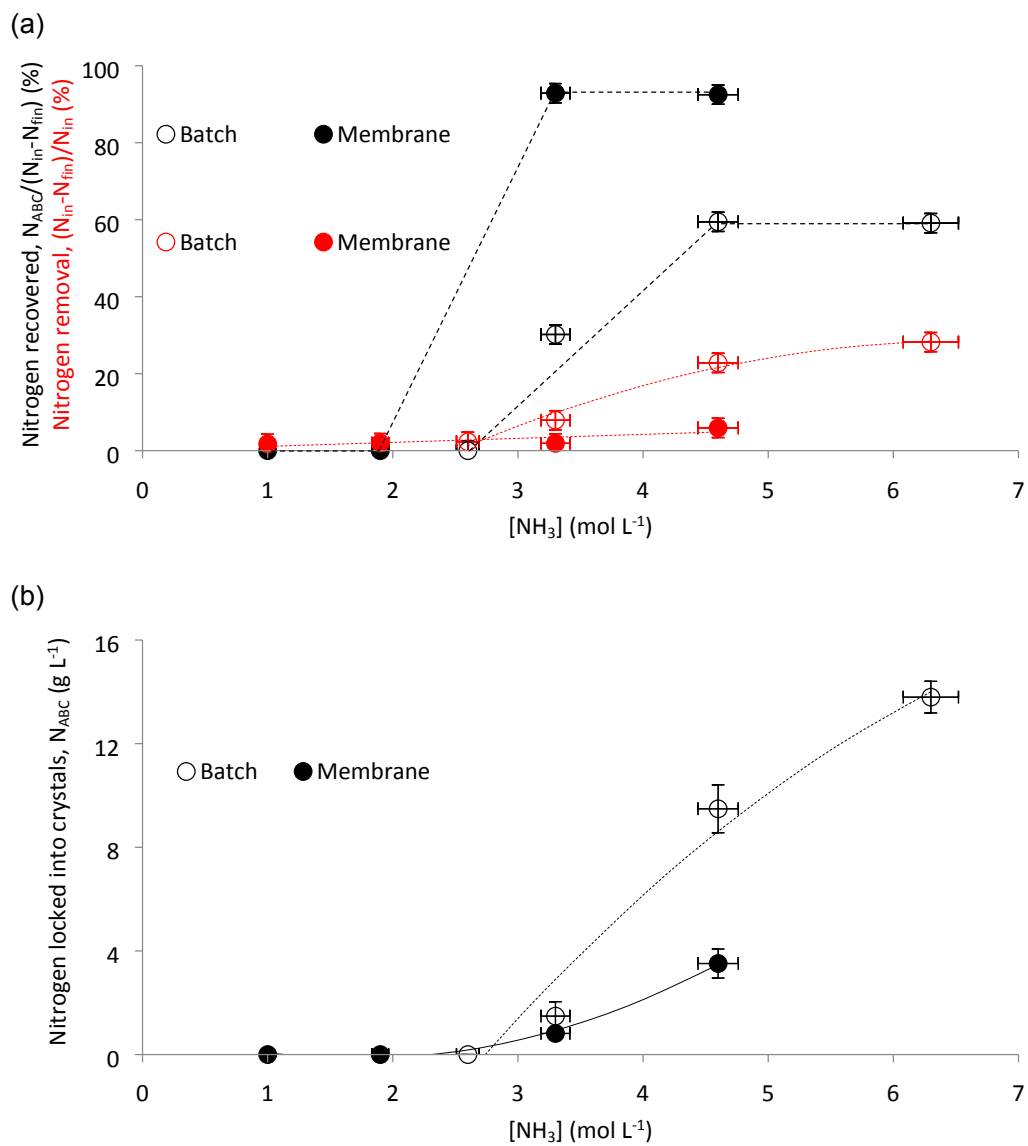
Figure 7. (a) Impact of aqueous ammonia concentration on ammoniacal nitrogen removal, calculated as (N_{\text{in}} - N_{\text{fin}})/N_{\text{in}} (%), where N_{\text{in}} and N_{\text{fin}} are initial and final ammoniacal nitrogen concentrations (g L -1 ) (red data points), and recovered, calculated as N_{\text{ABC}}/(N_{\text{in}} - N_{\text{fin}}) (%) (black data points), where N_{\text{ABC}} is nitrogen concentration locked into the crystals (g L -1 , figure b). Liquid volumes: 0.2L and 0.15L for batch and membrane operation, respectively. Error bars indicate standard deviation obtained from sacrificial experiments carried out in triplicate.
