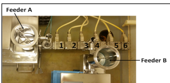
Figure 2: Twin screw extruder, consisting of six heating sections with two attached volumetric feeders (A and B).
