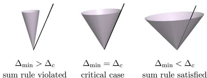
Figure 6: The three geometric situations described in the text. The thick black line denotes the vector corresponding to the function F \equiv 1 .
