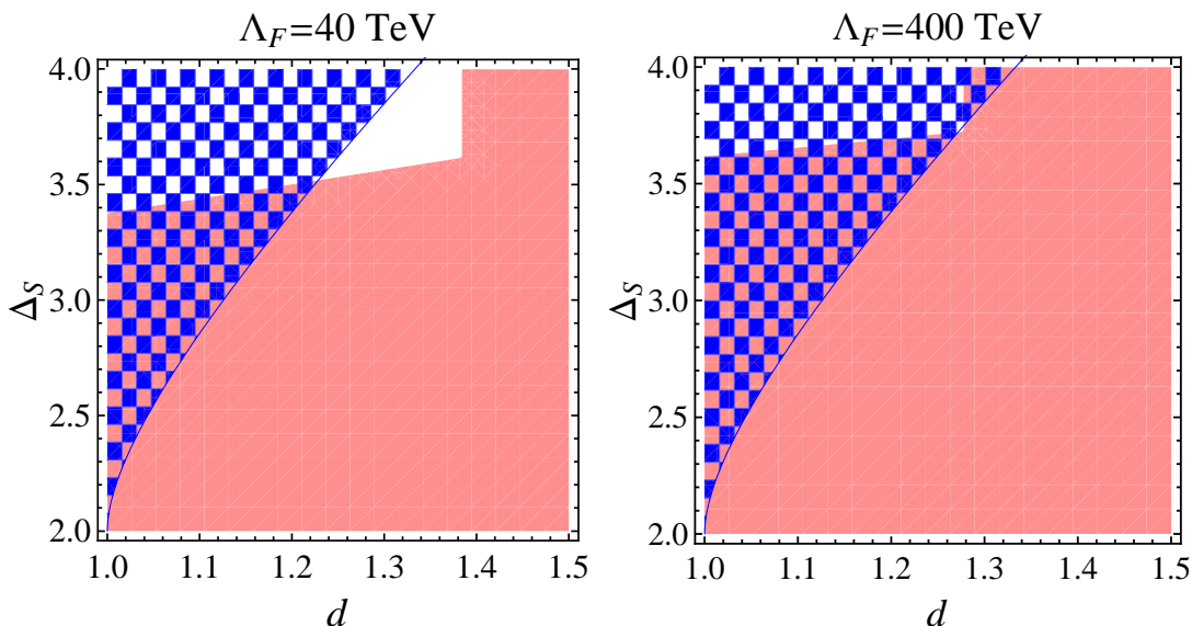
Figure 16: Solid red: The region of (d, \Delta_S) plane disfavored by phenomenological considerations of section 2. In this region one or both constraints (2.21), (2.22) are not satisfied. We consider two cases: \Lambda_F = 40 \text{ TeV} (left) and \Lambda_F = 400 \text{ TeV} (right). Checkered blue: the region of the same plane which would be excluded by our bound (1.4) with f = f_6 if we knew that \Delta_S < \Delta_T .
