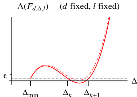
Figure 12: Solid curve: schematic typical dependence of the functional \Lambda(F_{d,\Delta,l}) on \Delta . The functional \Lambda satisfies (5.15) for all \Delta from a discrete trial set, which includes the dimensions \Delta_k and \Delta_{k+1} = \Delta_k + \delta\Delta . Yet the functional may become slightly negative for \Delta_k < \Delta < \Delta_{k+1} . Dashed curve: same for a functional corresponding to a smaller \delta\Delta . The violation of (5.13) at intermediate values has disappeared.
