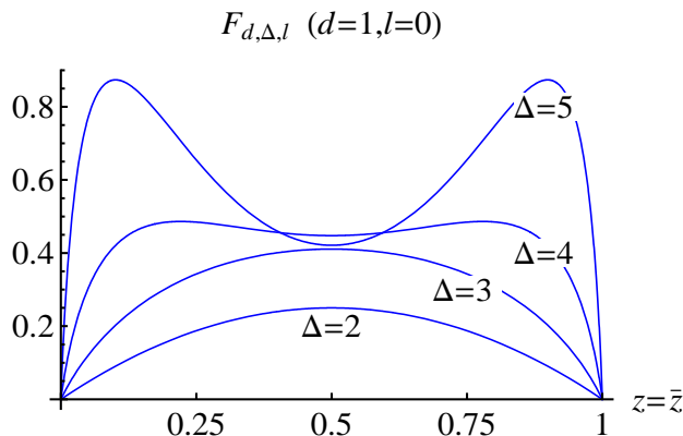
Figure 5: Same as figure 4, for l = 0 .
