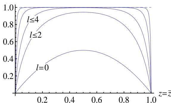
Figure 3: The r.h.s. of the sum rule in the free scalar theory, summed over l \leq 0, 2, 4, 8, 16 (from below up) and plotted for 0 \leq z = \bar{z} \leq 1 . The asymptotic approach to 1 (dashed line) is evident. Notice the symmetry with respect to z = 1/2 , a consequence of (4.7).
