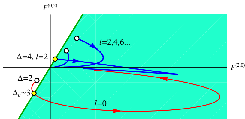
Figure 9: The analogue of figure 8 for d = 1.05 . In this plot we started the l = 0 curve at \Delta = 2 . The green line is the boundary of the projected cone for \Delta_{\min} = \Delta_c \simeq 3 , see figure 10. The slope of this line is determined by the energy-momentum tensor vector.
