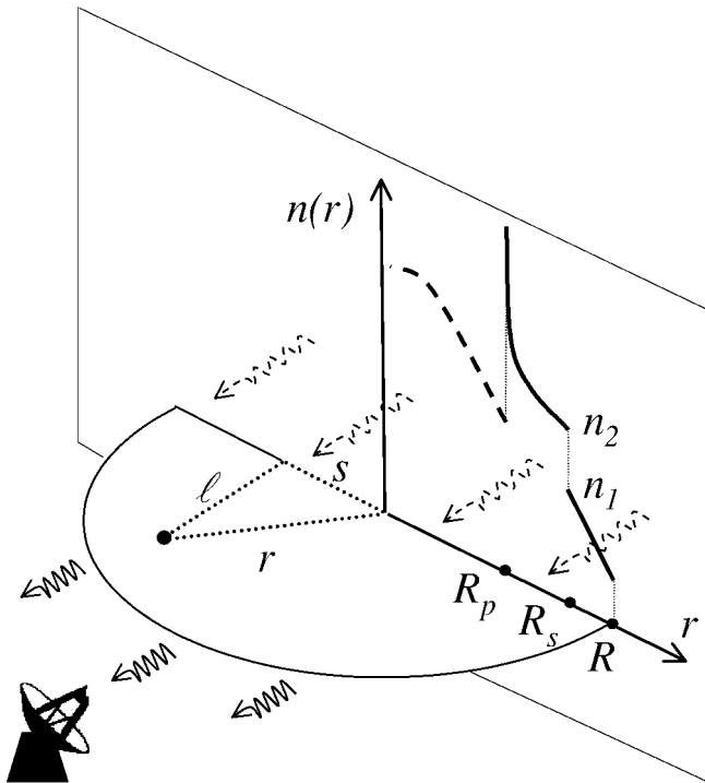
FIG. 1.—Geometry underlying eq. (1). For a point in the structure, r is the radial coordinate, s is its projection on the plane of the sky, and l is the coordinate along the line of sight. On the vertical axis, we outline the initial density run and the flow perturbed by the AGN-driven blast wave.
