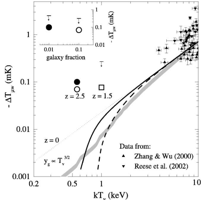
FIG. 3.—Predicted SZ signals as a function of the virial temperatures of galaxies, groups, and clusters. Dotted line : Baseline y_g at z = 0 . Shaded strip : Central signals from gas in the equilibrium set by SN preheating (Cavaliere & Menci 2001). Thick lines : Same for feedback from AGNs with M_{\text{BH}} = 10^9 M_\odot and coupling f = 3 \times 10^{-2} ( solid line ) or f = 10^{-1} ( dashed line ). Square : Area-averaged undiluted signal from a group at z = 1.5 , driven by AGN activity with M_{\text{BH}} = 10^9 M_\odot and f = 5 \times 10^{-2} ; the bar represents the bound for \omega = 2.4 . Circles : Same from a massive galaxy at z = 2.5 , for \Delta E = E ( open ) or 3E ( filled ); the inset specifies the statistics.
