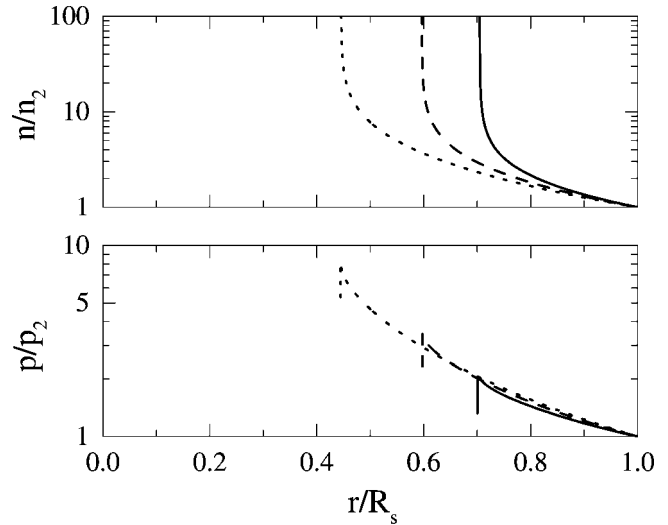
FIG. 2.—Radial distribution of density and pressure in the blast wave, relative to the postshock values n_2 and p_2 . Solid lines : Strong shock with \Delta E/E = 3 ; dashed lines : intermediate shock with \Delta E/E = 1 ; dotted lines : weak shock with \Delta E/E = 0.3 . The corresponding piston positions are given by \lambda \approx 0.7, 0.6 , and 0.45 .
