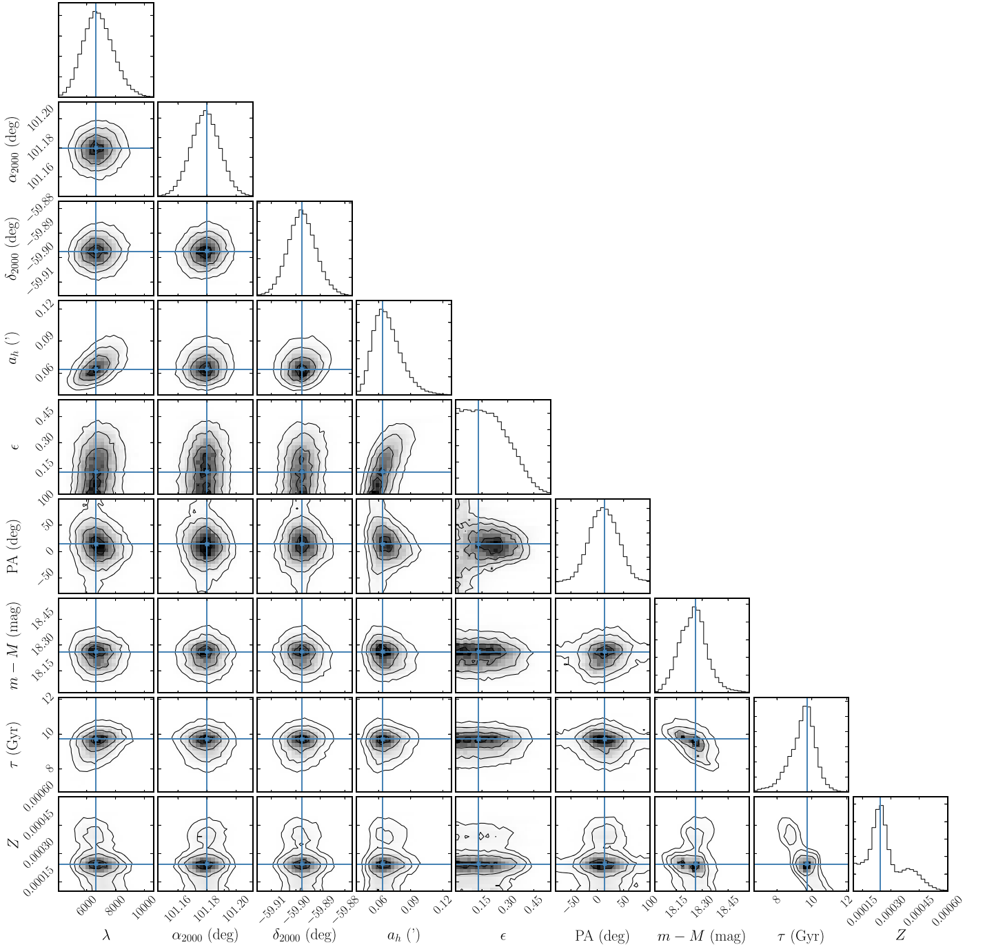
Figure 3. Posterior probability densities from a nine-parameter maximum-likelihood fit of MagLiteS J0644–5953 (Pic II). From left to right the nine parameters are as follows: stellar richness ( \lambda ), right ascension ( \alpha_{2000} ), declination ( \delta_{2000} ), semimajor half-light radius ( a_h ), ellipticity ( \epsilon ), position angle (P.A.), distance modulus ( m - M ), age ( \tau ), and metallicity ( Z ). The crosshairs indicate the best-fit parameter values from a kernel density estimate of the peak of the posterior distribution.
