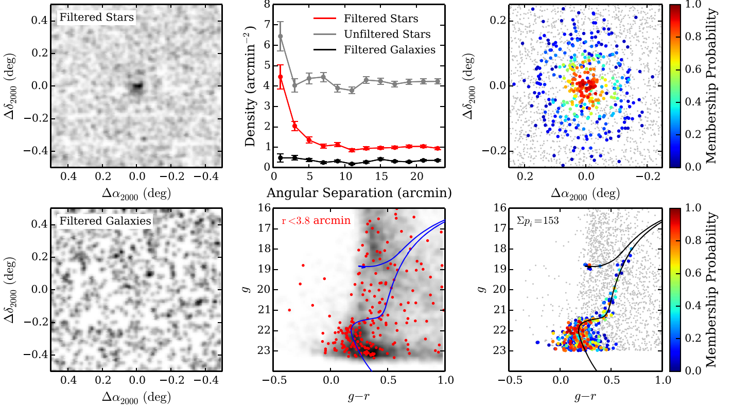
Figure 2. Stellar density and color–magnitude diagrams for (Pic II). Top left: spatial distribution of stars with g < 24 mag that pass the isochrone filter (see the text). The field of view is 1^\circ \times 1^\circ centered on the candidate and the stellar distribution has been smoothed by a Gaussian kernel with standard deviation 0.6 . Top center: radial distribution of objects with g - r < 1 mag and g < 24 mag: stars passing the isochrone filter (red), stars excluded from the isochrone filter (gray), and galaxies passing the isochrone filter (black). Top right: spatial distribution of stars with high membership probabilities within a 0.5^\circ \times 0.5^\circ field of view. Gray points indicate stars with a membership probability less than 5%. Bottom left: same as the top left panel, but for galaxies passing the isochrone filter. Bottom center: the color–magnitude distribution of stars within r = 3.8 of the centroid are indicated with individual points. The density of the field within an annulus 0.5 < r < 1.0 is represented by the background grayscale. The blue curve shows the best-fit isochrone as described in Section 4 and Table 1. Bottom right: color–magnitude distribution of high membership probability stars.
