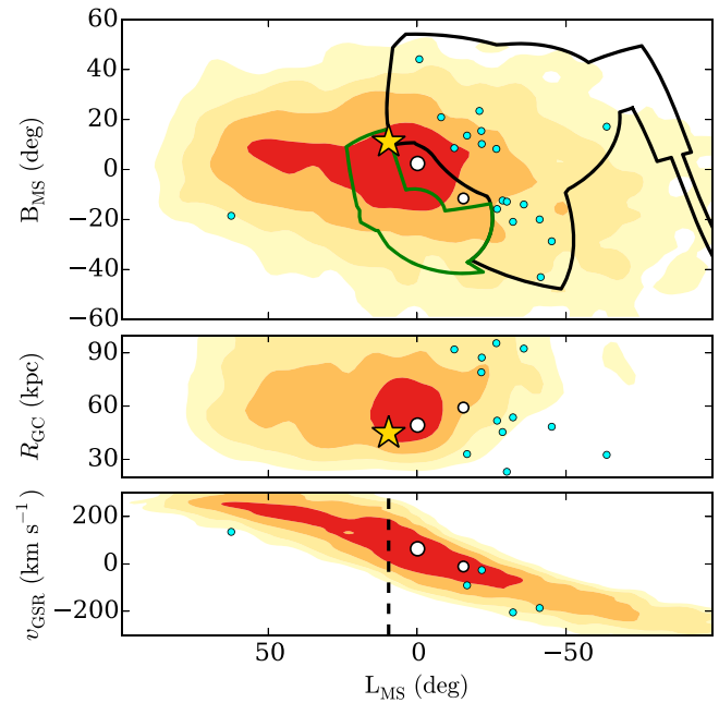
Figure 4. Phase space coordinates of MagLiteS J0644–5953 (Pic II) (gold star) relative to the simulated distribution of LMC satellites from Jethwa et al. (2016), represented by colored contours. Recently discovered DES satellites and Hydra II are shown with cyan markers. Top: the density of simulated LMC satellites projected onto the sky in MS coordinates. The DES and MagLiteS footprints are outlined in black and green, respectively. Middle: the density of simulated LMC satellites with 5^\circ < B_{\text{MS}} < 25^\circ projected onto the plane of Galactocentric radius and MS longitude. Bottom: distribution of line-of-sight velocities in the Galactocentric standard reference frame for simulated satellites of the LMC. The black dashed line represents the MS longitude of MagLiteS J0644–5953 (Pic II). The figure is adapted from Jethwa et al. (2016).
