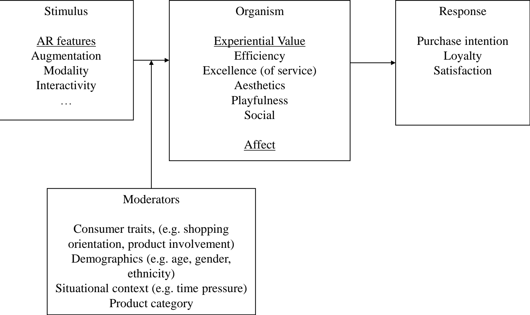
Figure 3 Proposed framework
