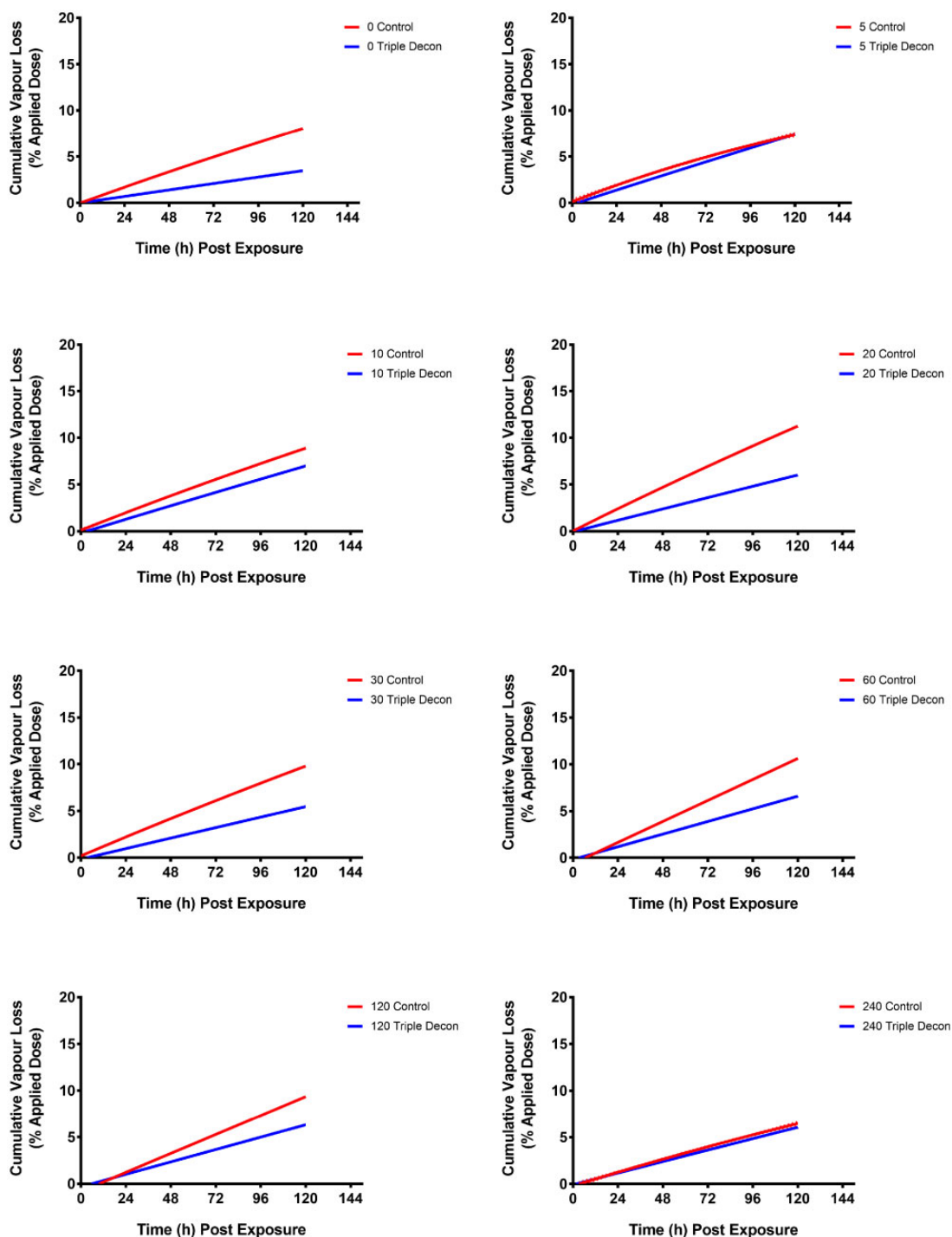
Figure 4. Percentage of applied dose of ^{14}\text{C} -phorate expressed as cumulative vapor loss from human hair over 120 h (6 hourly intervals). Each swatch of human hair was exposed to a 20\ \mu\text{l} droplet of ^{14}\text{C} -PHR and subjected to either no decontamination (control) or decontamination using combined dry, ladder pipe system, and technical decontamination (triple protocol) at 0, 5, 10, 20, 30, 60, 120, and 240 min postexposure.
