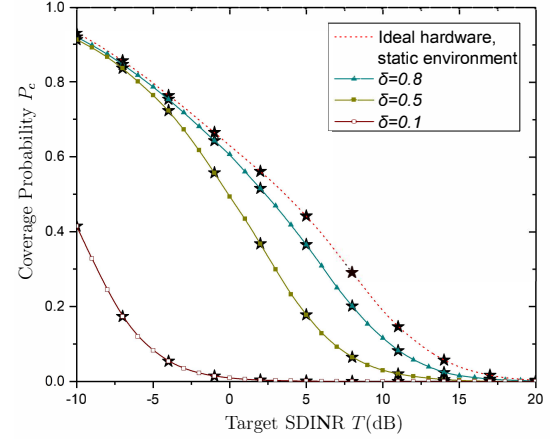
Fig. 1. Coverage probability of a MU-MIMO mmWave HetNet versus the target SDINR T for varying severity of channel aging, while the RATHIs and ATN are assumed to have no impact ( \kappa_{tBS} = \kappa_{rUE} = 0 , \xi = \sigma^2 ).
