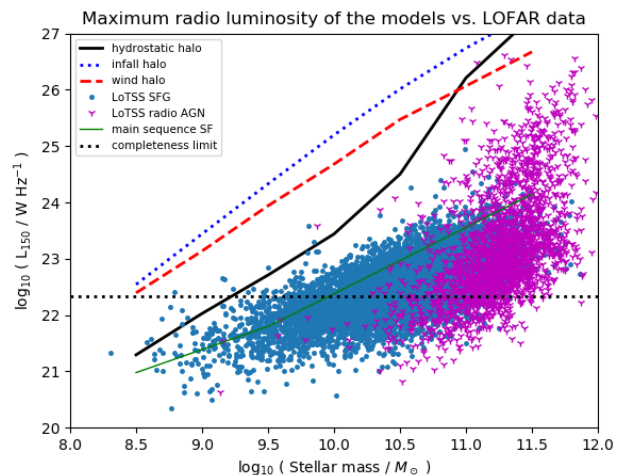
Fig. 3. Maximum 150 MHz luminosity of radio AGN for a given galaxy mass for three different models of the gaseous halo of the galaxies (hydrostatic halo, infall halo, wind halo). Data points are from the LoTSS sample (Sabater et al. 2019), plotted separately for star forming galaxies (SFG) and radio AGN. The radio luminosity expected from star formation for galaxies on the main sequence of star formation at redshift zero is indicated as solid thin green line (Sect. 2.3, eq. (3) in Gürkan et al. 2018). The dotted black line denotes the completeness limit, i.e., the median limiting luminosity at the maximum redshift of the sample. For the hydrostatic halo model, radio AGN with the same Eddington-scaled jet power distribution could be hosted by galaxies of all masses. The lower densities in the halos of lower mass galaxies would, however, limit their radio luminosities. Radio AGN need to be intrinsically less powerful or otherwise different in low mass galaxies that are in galactic wind or (any) quasi-spherical infall phases in order not to exceed the LOFAR radio luminosity constraints.
