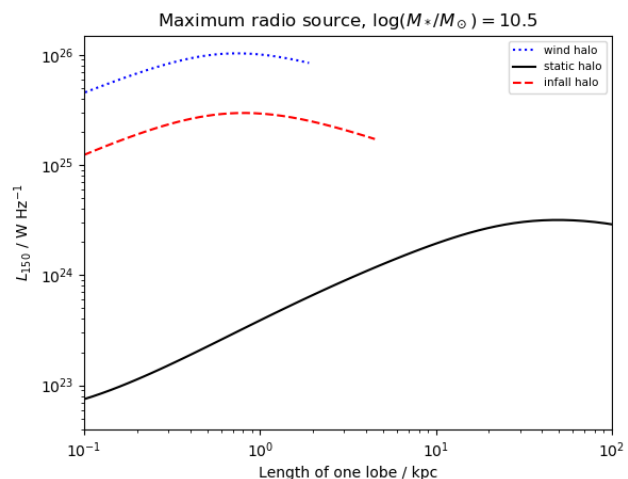
Fig. 2. Example radio luminosity at 150 MHz versus lobe length plots for hydrostatic, galactic wind and infall halos for a galaxy of stellar mass M_* = 3 \times 10^{10}M_{\odot} and the maximum plausible jet power in our model of 2 \times 10^{36} W. See Sect. 2 for details of the gaseous halo models and Sect. 3 for details of the radio source model.
