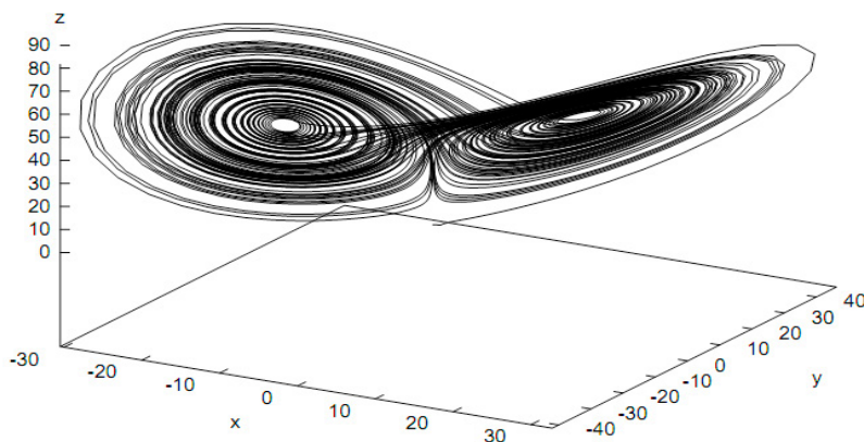
Figure 2. A visualisation of the Lorenz attractor in 3-dimensional phase space x(t), y(t), z(t) [7].
