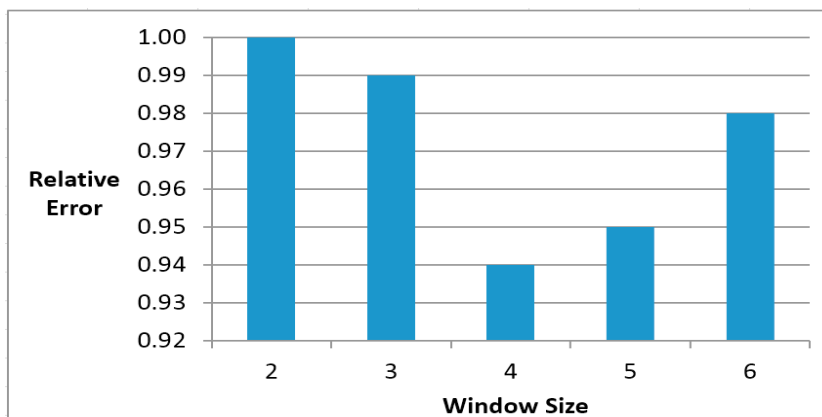
Figure 5. Relative error of the predictor for varying window size for HRV Time series.
