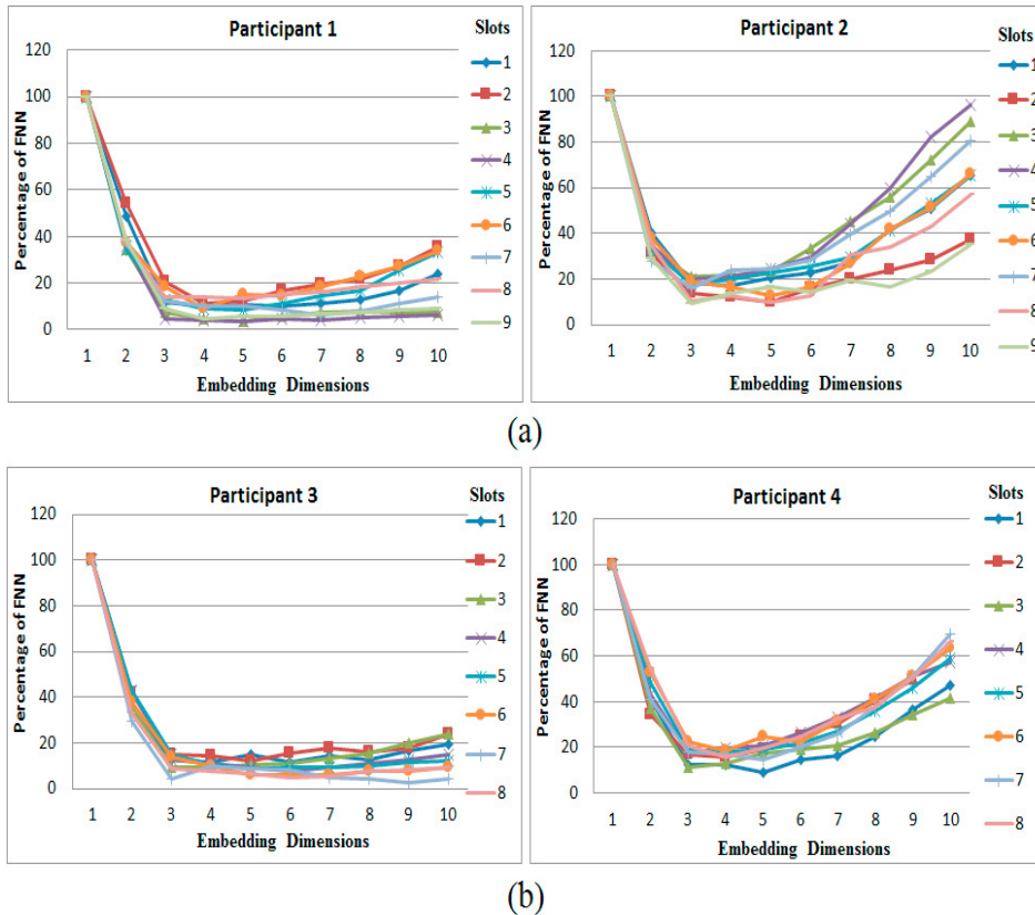
Figure 4. Embedding Dimension Result: (a) Two participant's (Participant 1 and 2) ED result from Dataset 1, and (b) Two participant's (Participant 3 and 4) ED result from Dataset 2.
