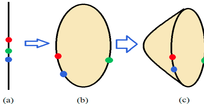
Figure 1. Geometric explanation of the FNN Algorithm [8]: (a) In one-dimensional, Red and Green Point are nearest neighbour, (b) In two-dimensional Red and Green point are not nearest neighbour (i.e. false nearest neighbour), but Red and Blue are nearest neighbour, and (c) In three-dimensional Red and Blue are still nearest neighbour, so they are real nearest neighbour.
