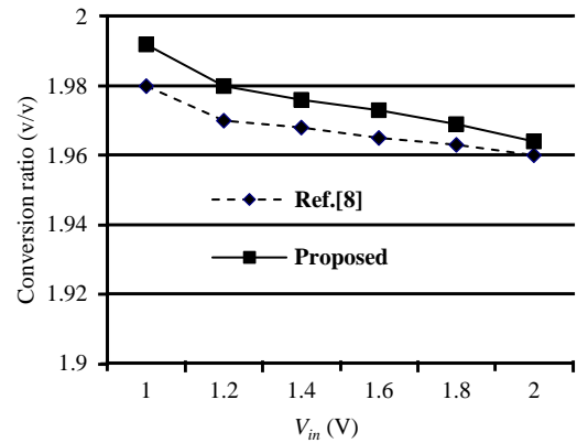
Fig. 9. Voltage conversion ratio versus supply voltage.
