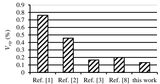
Fig. 10. Output ripple voltage comparison.
