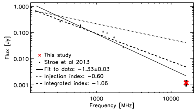
Figure 2. Integrated radio spectrum of the northern relic from 153 MHz up to 16 GHz (see also Table 1). The red cross marks the 16 GHz measurement. The uncertainties include a 10 per cent flux scale error added in quadrature to the \sigma_{\text{RMS}} . A power-law is fitted to the eight frequencies. The dotted line shows the injection spectrum and the dashed line the integrated spectrum, as derived from high-resolution GMRT and WSRT data (Stroe et al. 2013). The injection and integrated spectra below 2.3 GHz are consistent with a CI model. The 16 GHz measurement is 12\sigma below the CI prediction.
