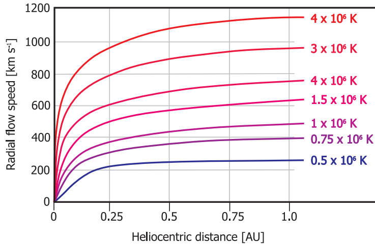
Figure 1: Solutions to the Parker solar-wind equation (described in Section 2) for a range of coronal temperature and heliocentric distance, in astronomical units (AU). Adapted from [65].
