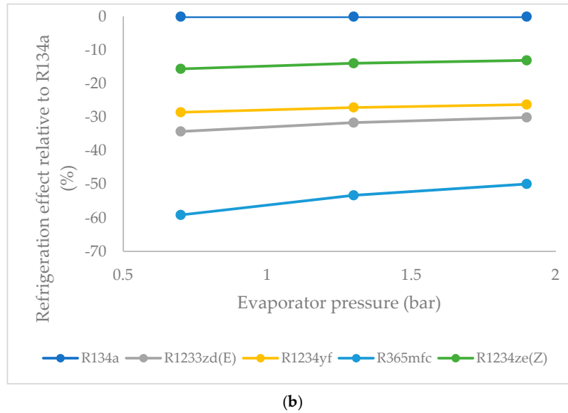
Figure 7. (a) Refrigeration effect as a function of evaporator pressure (condenser pressure = 9 bar). (b) Refrigeration effect relative to R134a (condenser pressure = 9 bar).
