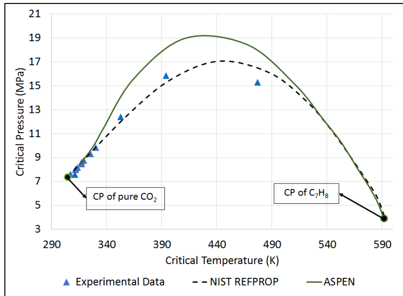
Figure 2: Critical loci of \text{CO}_2 -Toluene binary mixture in P - T plane. The experimental data is taken from 41,43 .
