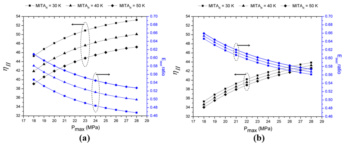
Figure 5: Exergetic efficiency and exergy destruction ratio of (a) BSRC and (b) BPHC with respect to cycle maximum pressure and minimum temperature difference inside the recuperator (MITA R ).
