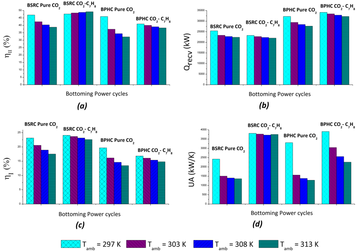
Figure 11: Thermodynamic comparison of bottoming power cycles operating with \text{CO}_2\text{-C}_7\text{H}_8 and pure \text{CO}_2 as working fluids at four ambient temperature conditions.
