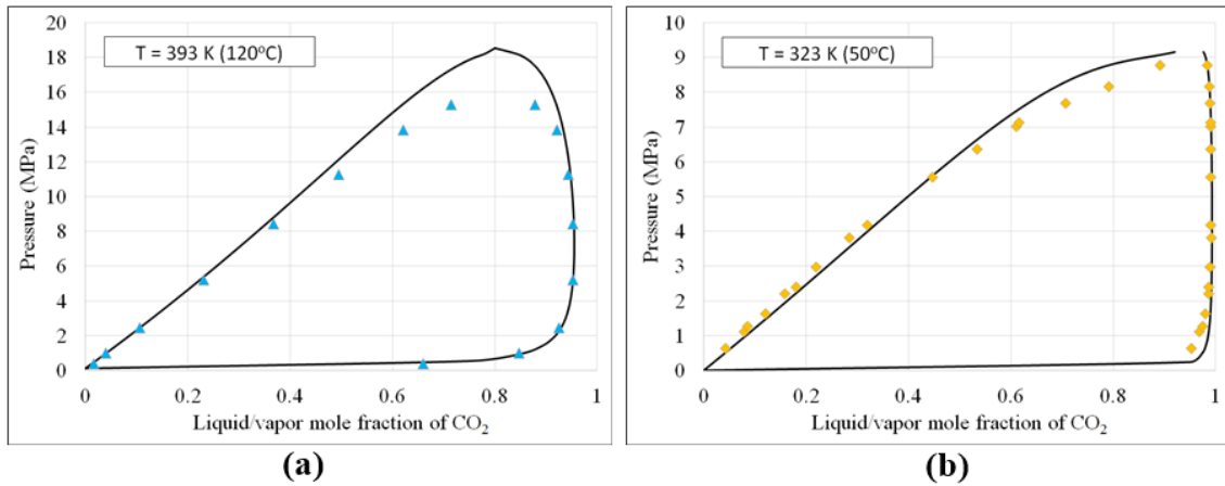
Figure 1: VLE of CO 2 -Toluene binary mixture at (a) T=393\text{ K} and (b) T=323\text{ K} computed using PR EoS in Aspen Plus. The experimental data taken from 41,42 .
