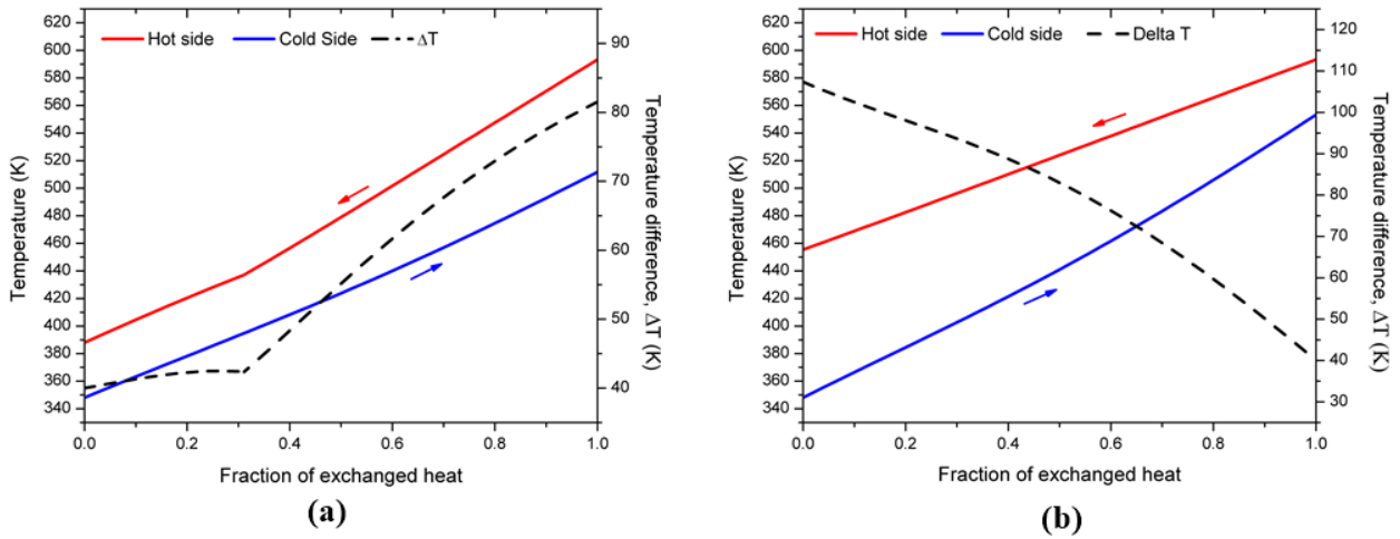
Figure 8: Temperature-heat exchange ( T-Q ) curves of recuperator in (a) BSRC and (b) BPHC. Hot stream corresponds to stream coming from turbine side while cold stream corresponds to stream coming from compressor side. Dotted lines show temperature difference between the two streams.
