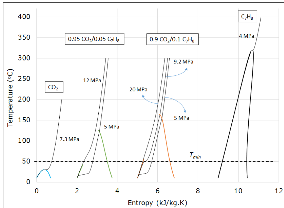
Figure 3: T - s diagram of \text{CO}_2 , Toluene and their binary mixtures at two compositions. This figure is adapted from 17 .
