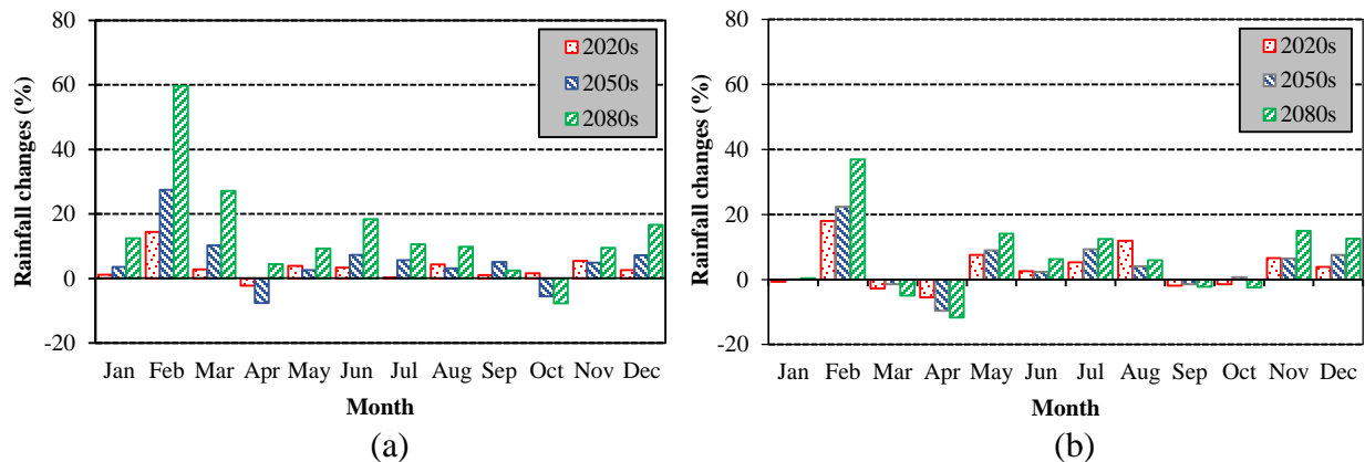
Fig. 2 Mean monthly rainfall changes for the decades of 2020s, 2050s and 2080s in comparison to the baseline period under (a) A2 scenario and (b) B2 scenario
