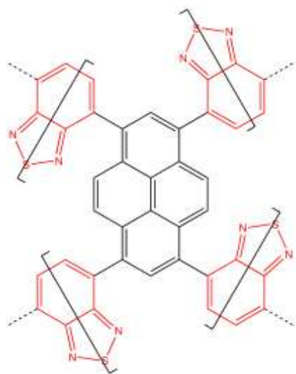
BTZ-Py polymer
