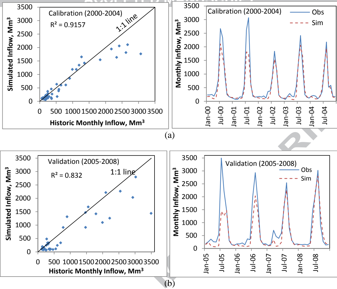
Fig. 7 Comparison of observed and simulated monthly river flow during: (a) calibration; and (b) validation
