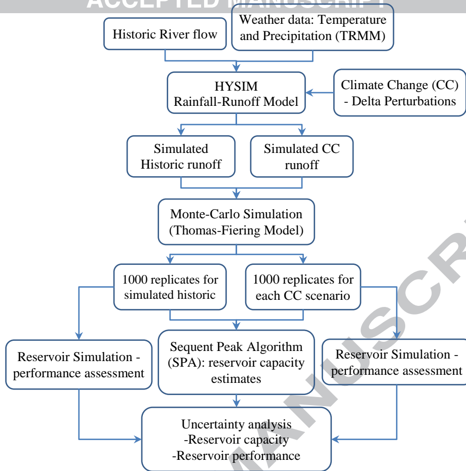
Fig. 2 Methodology flow chart
