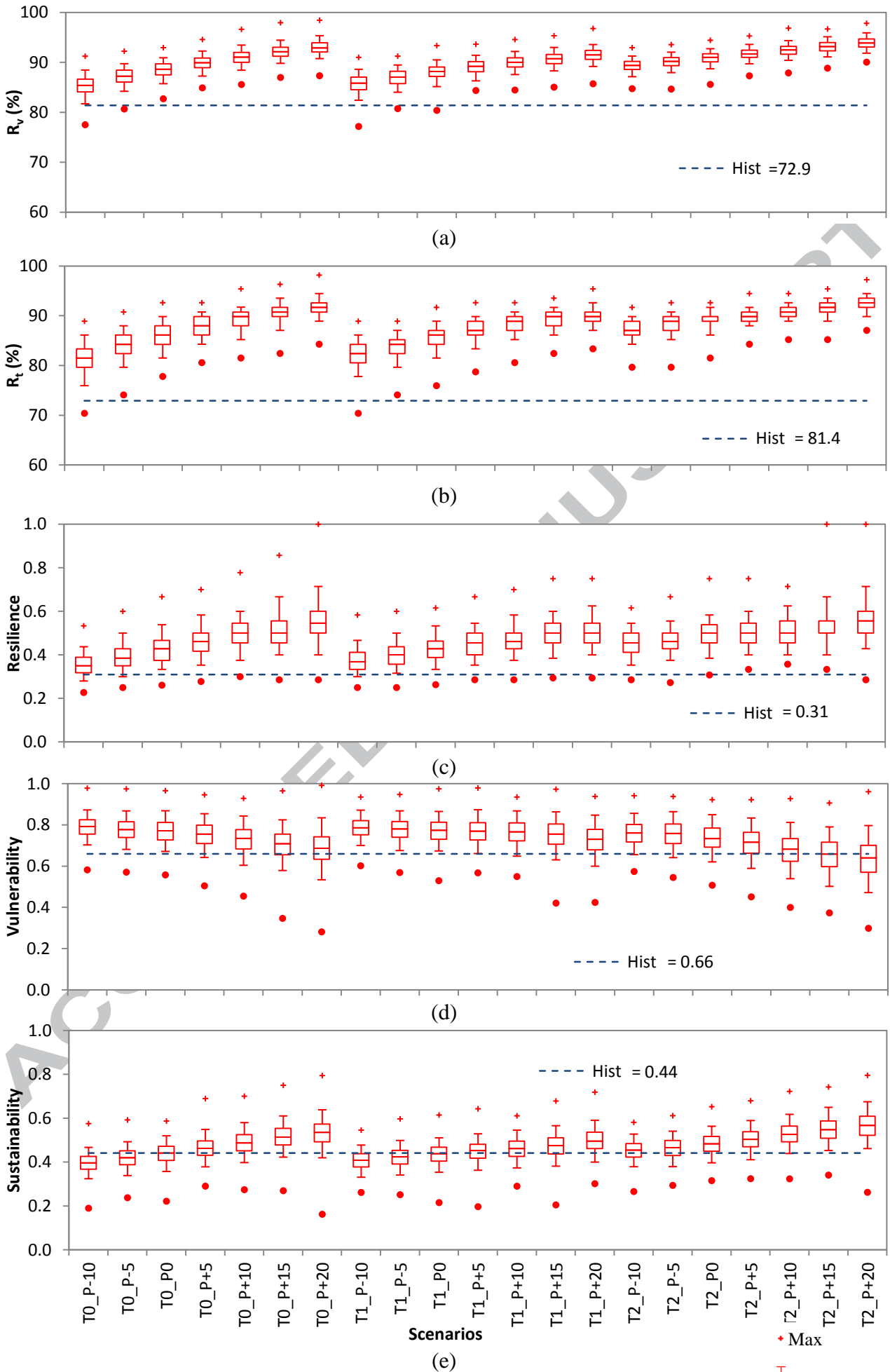
Fig. 11 box plot of reservoir performance: (a) Volume reliability; (b) Time reliability; (c) Resilience; (d) Vulnerability; (e) Sustainability (based on R_t )
