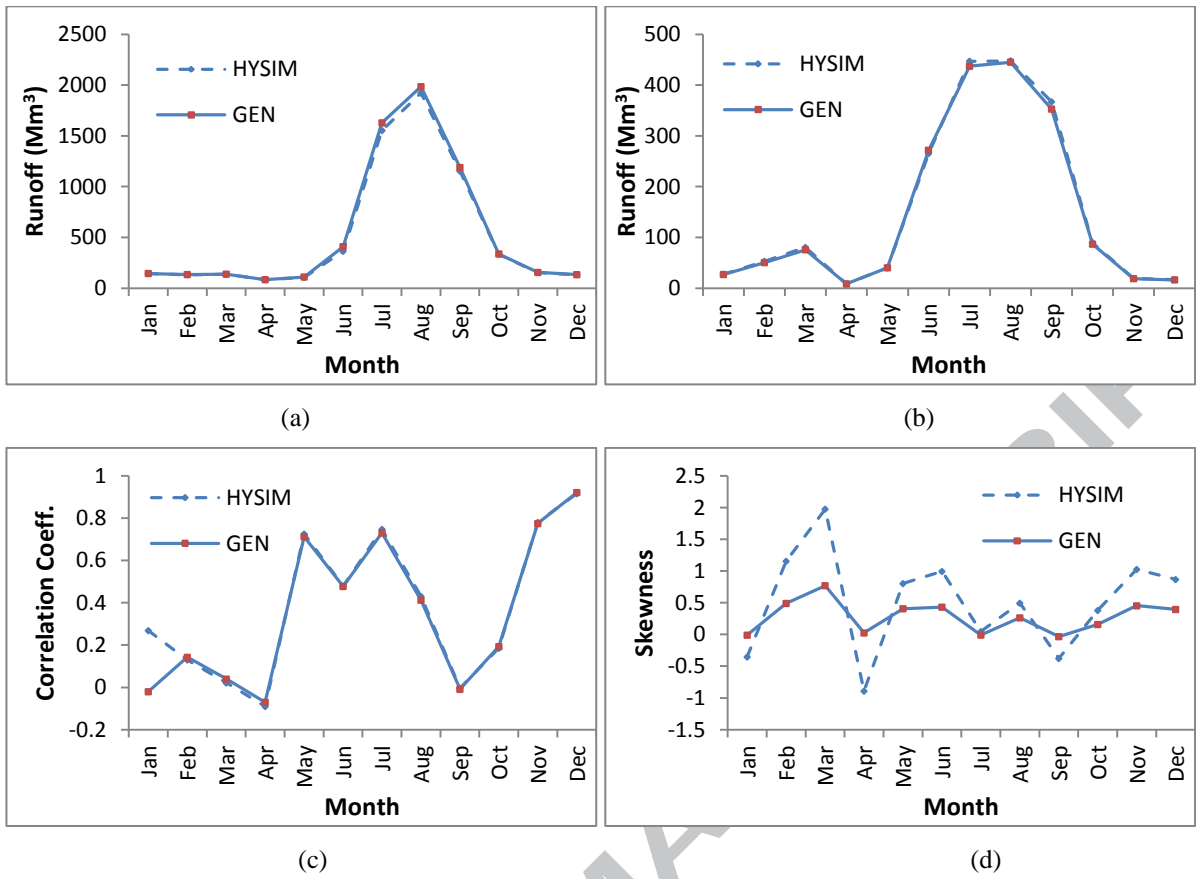
Fig. 9 Comparison of statistics of 'observed' (HYSIM) and stochastically generated (GEN) runoff: (a) mean; (b) standard deviation; (c) correlation coefficient; and (d) skewness
