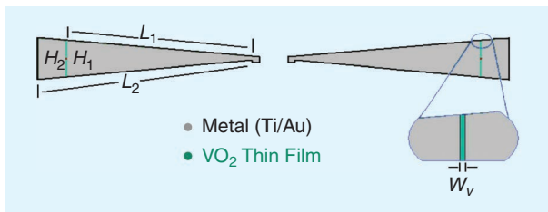
FIGURE 9. The layout of a reconfigurable bowtie antenna with VO 2 (turquoise) on both arms [47]. The VO 2 strips are only 20- \mu\text{m} wide. The measured gain patterns at the heated (4.58-GHz) and unheated (4.72-GHz) states showed they vary minimally, as expected for a frequency-tunable antenna.
