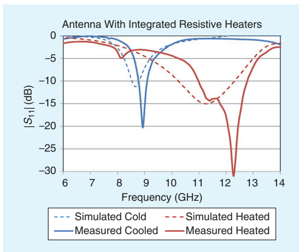
FIGURE 20. The measured and simulated |S_{11}| of the VO 2 antenna with integrated resistive heaters, demonstrating a large frequency shift when the VO 2 is heated.
