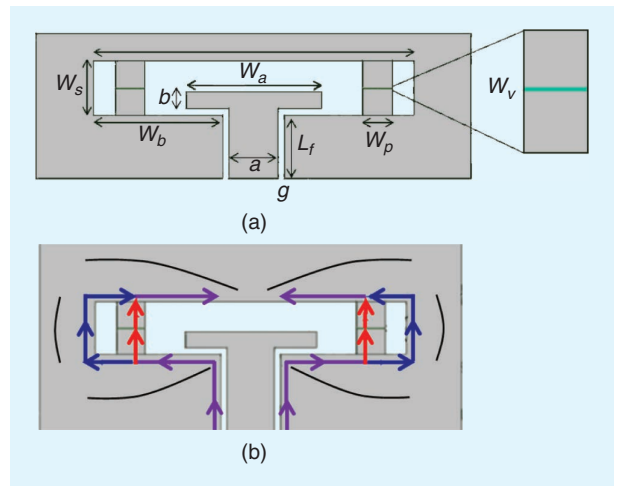
FIGURE 11. (a) The layout (not to scale) of a reconfigurable folded slot with the VO 2 (turquoise) strips on both paths reducing its circumference upon activation. (b) The operating principle of the antenna, showing the directions of the currents in each configuration (blue/red) and the standing wave of the current (black).
