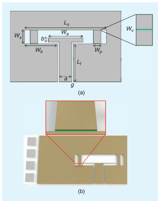
FIGURE 16. A folded aperture antenna with four VO 2 thin-film strips. (a) The 2D plot, top view. (b) The 3D plot showing the VO 2 and metallization layers in scale.
