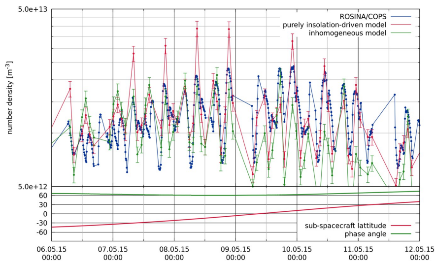
Fig. 9. Model fits to the ROSINA/COPS data (blue dots) with insolation-driven (red dots) and inhomogeneous models (green dots). The quality of the comparisons is in both cases reasonably good with the inhomogeneous distribution providing a slightly better fit to the data. The sub-spacecraft latitude and phase angle are shown in the lower panel.
