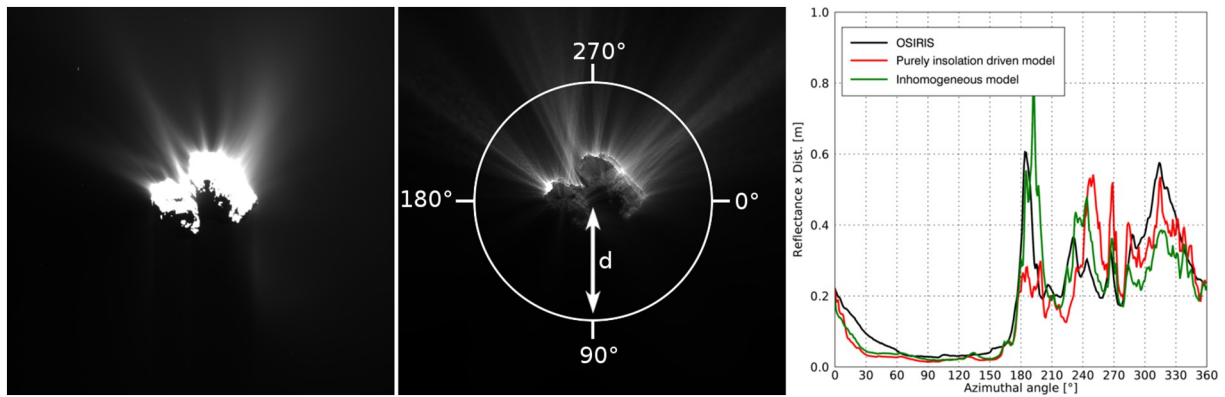
Fig. 18. Left panel: Stretched and cropped OSIRIS-WAC image taken on 2015-05-05 09:27:54 UTC. Centre panel: Modelled dust brightness for the inhomogeneous model. Right panel: Reflectance multiplied by the projected distance from the nucleus centre (impact parameter, d ) as a function of azimuthal angle (AZ) on circle around the nucleus as indicated in the centre panel. The curves show the OSIRIS data (black line), the purely insolation-driven model (red line) and the inhomogeneous model (green line). Here d = 2.5 km.
