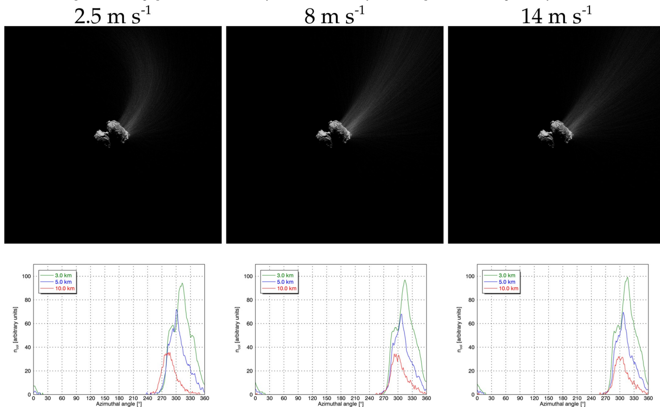
Fig. A.22. The top row shows the dust column density, n_d, \text{ol} , for three different initial speeds ( 2.5 \text{ m s}^{-1} , 8 \text{ m s}^{-1} , and 14 \text{ m s}^{-1} ) of dust particles originating from the Imhotep region. The viewing geometry was chosen to be the one of the OSIRIS image of Fig. 18. The bottom row shows for each of the initial dust speeds the column density as a function of the azimuthal angle as in the right panel of Fig. 18.
