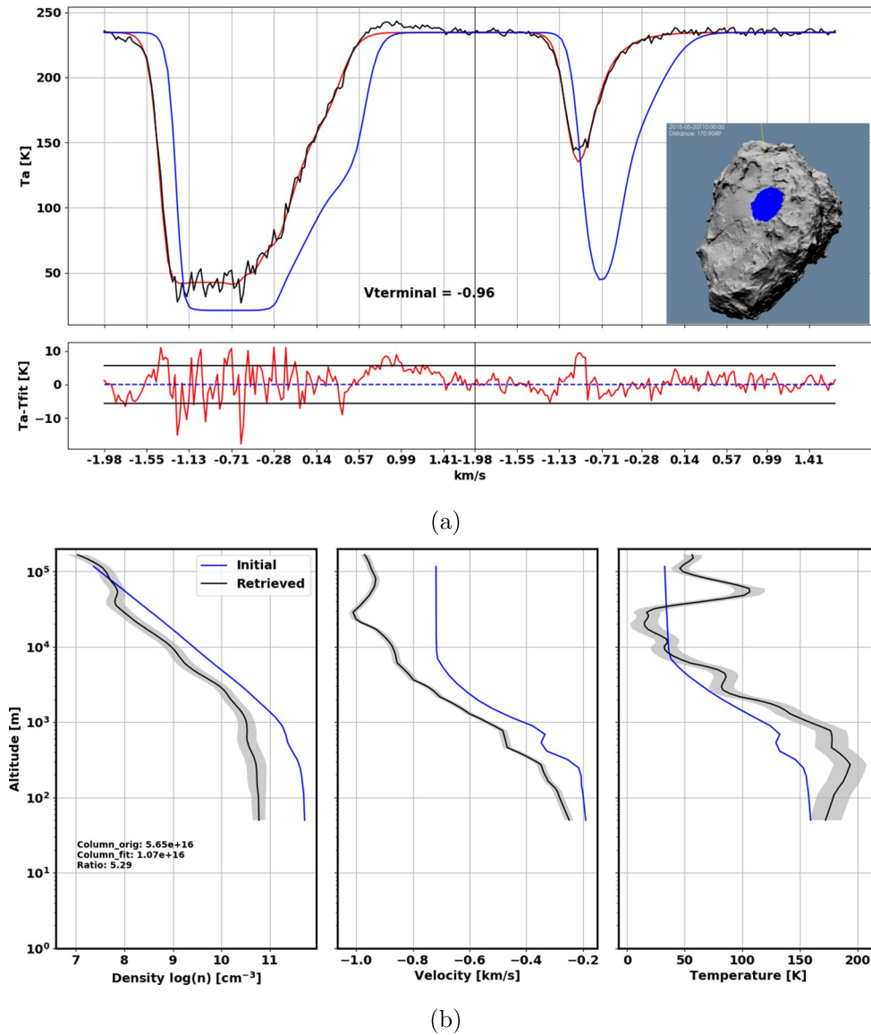
Fig. 17. Spectral lines and retrieved profiles for case D . The figure panels and colours have the same meaning as discussed in detail for case A . (a) Three spectra for the 557 GHz transitions of \text{H}_2^{16}\text{O} (left) and \text{H}_2^{18}\text{O} (right). (b) Vertical profiles of (left) number density, (middle) expansion velocity, and (right) kinetic temperature.
