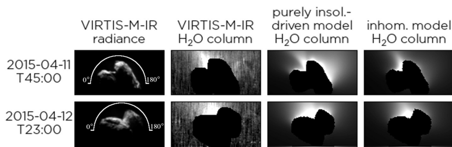
Fig. 10. Cubes a) and g) from Fig. 6 of Migliorini et al. (2016) are compared to our model. The top row shows cube a) data, and the bottom row shows cube g) data. The two left columns show the VIRTIS -M-IR radiance and the derived H 2 O column density. The 3rd column shows the modelled VIRTIS-M-IR H 2 O column density from the purely insolation-driven model. The 4th (rightmost) column shows the result from the inhomogeneous model.
