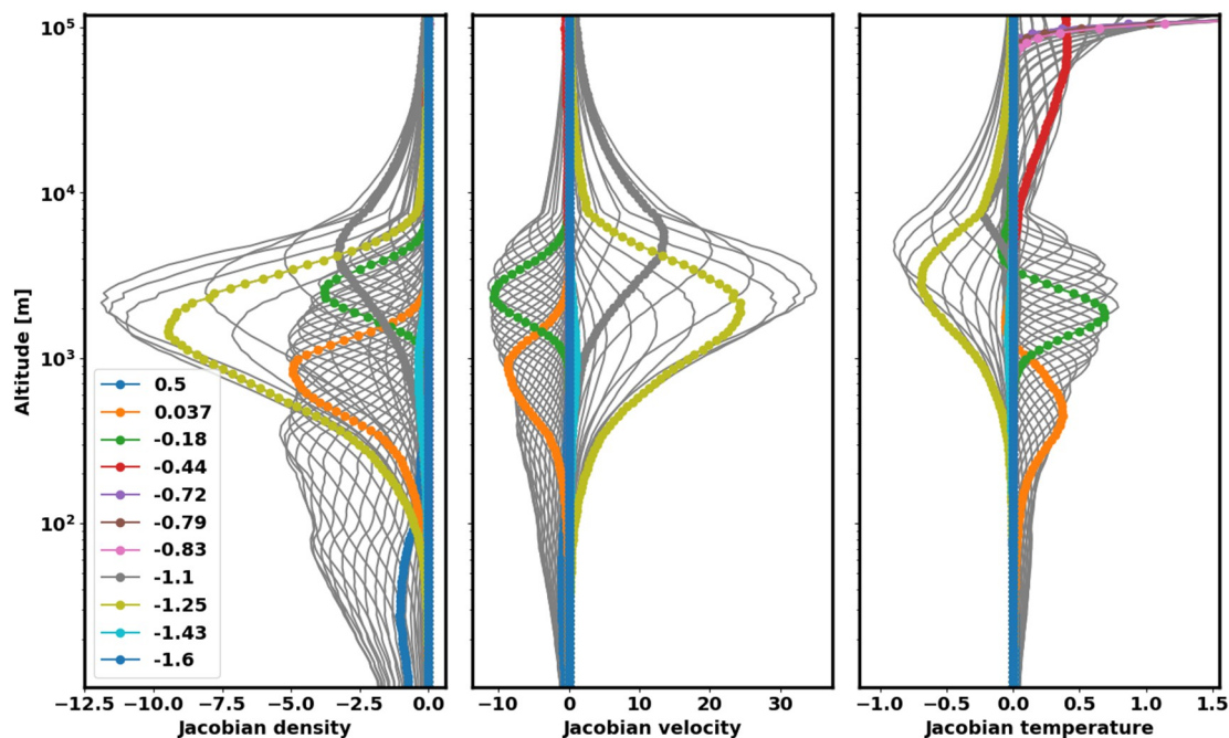
Fig. 5. The three panels show the Jacobians for the \text{H}_2^{16}\text{O} line with respect to density, expansion velocity, and temperature for a typical example of calculated profiles from the DSMC code. The lines in colour show rows of the Jacobian matrix for selected velocities (frequencies) shown in labels in units of [km/s] (in this example the line centre is at about -0.72 km/s). The abscissas are shown in arbitrary units.
