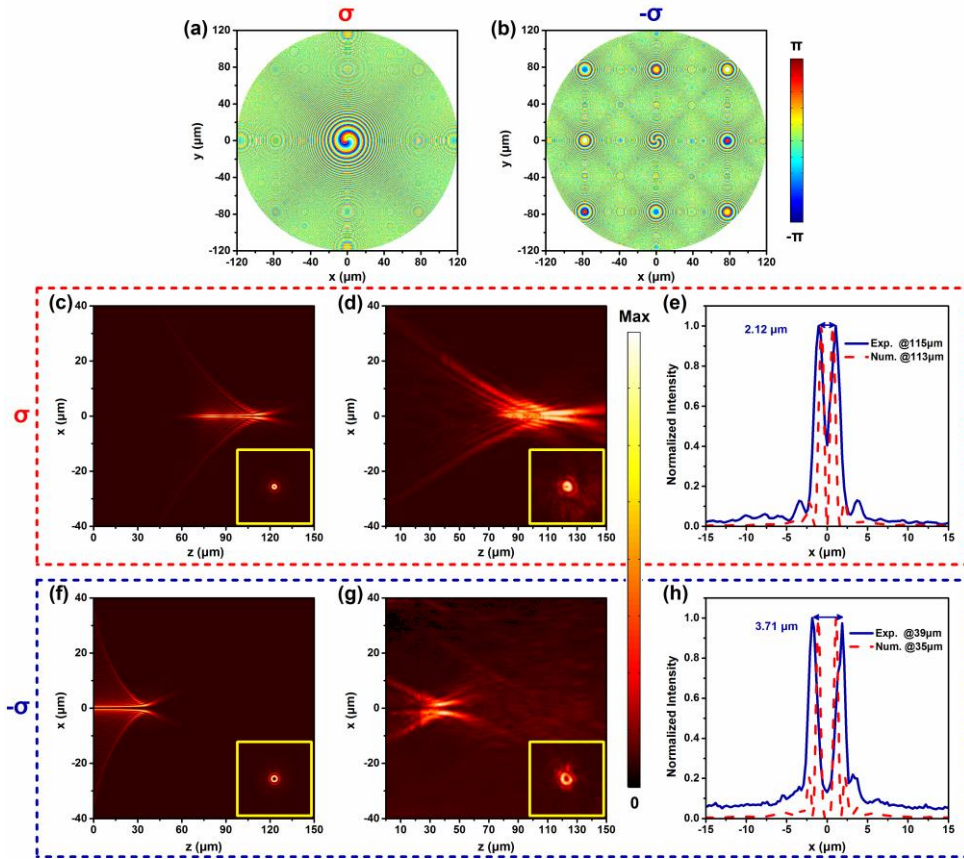
Figure 4. (Color online) Experimental demonstration of the SHG focusing optical vortex. Calculated phase profile for nonlinear focusing optical vortex with spin a) \sigma and b) -\sigma . Numerical intensity distributions along the propagation direction with spin c) \sigma and f) -\sigma , the insets show the intensity distributions at focal planes. Measured intensity distributions along the propagation direction with spin d) \sigma and g) -\sigma , the insets show the intensity distributions at focal planes. The numerical and measured
