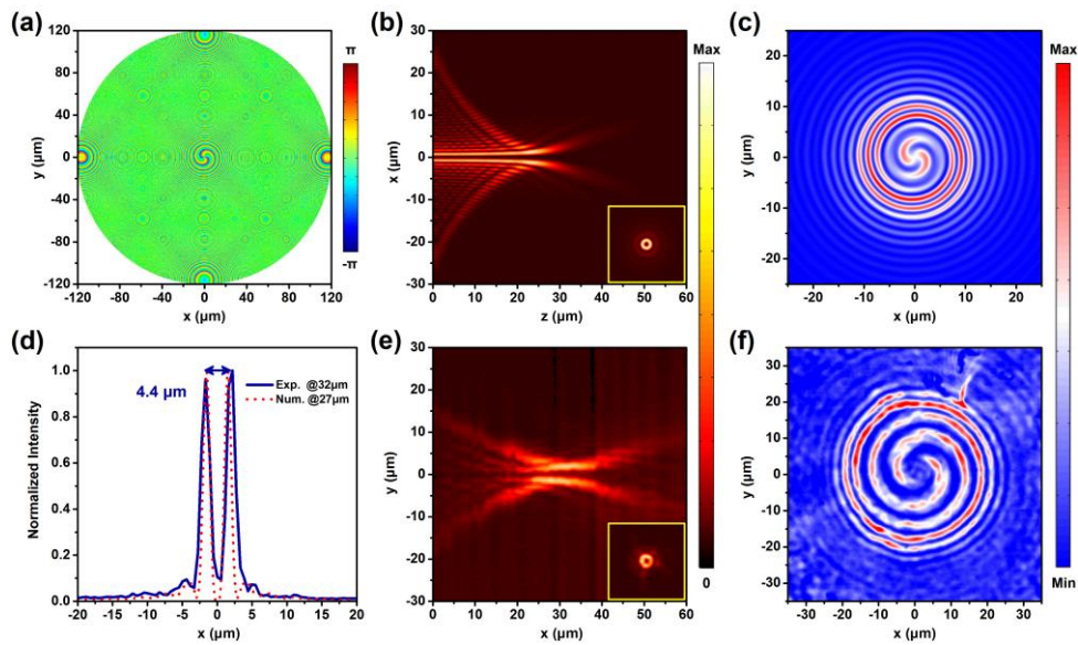
Figure 3. (Color online) Experimental demonstration of the linear focusing optical vortex. a) Calculated phase profile for linear focusing optical vortex with spin -\sigma . b) Numerical and e) measured intensity distributions along the propagation direction, the insets show the intensity distributions at focal planes. The scale bar is adapted for each figure. c) Numerical and f) measured interference patterns of the
