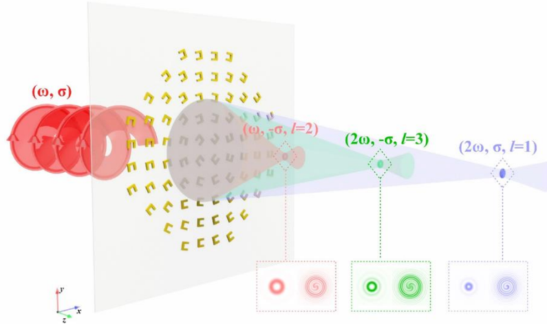
Figure 1. (Color online) Schematic of focusing optical vortices with proposed metasurface. With different combination of spin and wavelength, the three optical vortices with different topological charges focused at different focal planes. The insets show the numerical intensities and interference patterns of the optical vortices.
