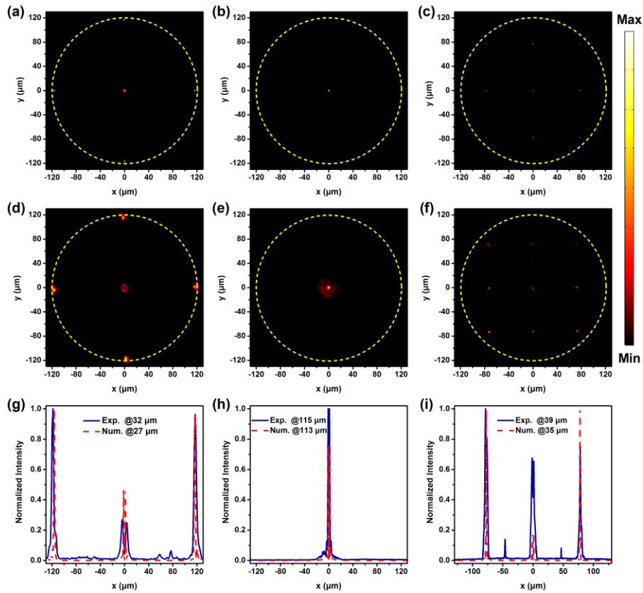
Figure 6. (Color online) Observation of multi-focal lenses. Numerical intensity distributions at focal planes of the linear focusing optical vortices with spin a) -\sigma , and SHG focusing optical vortices with spin b) \sigma and c) -\sigma . Measured intensity distributions at focal planes of the linear focusing optical vortices with spin d) -\sigma , and SHG focusing optical vortices with spin e) \sigma and f) -\sigma . The scale bar is adapted for each figure. The numerical and measured intensity cross profiles of the linear focusing optical vortex with spin g) \sigma and SHG focusing optical vortices with spin h) \sigma and i) -\sigma at focal planes.
