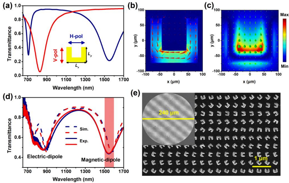
Figure 2. (Color online) Properties of the fabricated metasurface. a) Simulated transmission spectra for horizontal and vertical polarized incident light of uniformly arranged SRRs. Length of long arm L_x , short arm L_y , width w and thickness h of the nanoantenna are 167, 145, 40 and 35 nm, respectively. Characteristic snapshots of b) current density J and c) magnetic field B of an SRR at wavelength of 1550 nm. The scale bar is adapted for each figure. d) Simulated (dashed lines) and measured (solid lines) transmission spectra for horizontal and vertical polarized incident light of the fabricated metasurface for focusing optical vortices. The incident wavelengths are marked by a red stripe. e) SEM micrograph of a part of the fabricated metasurface. The set shows the whole metasurface with a radius of 120 \mu\text{m} .
