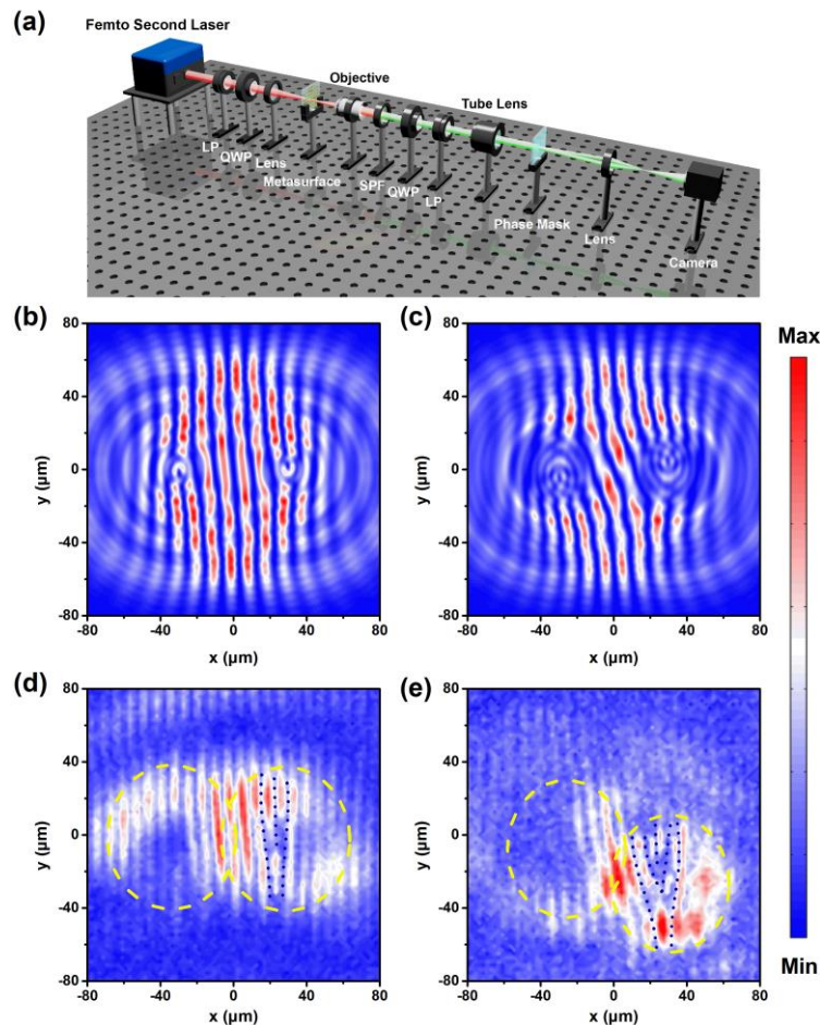
Figure 5. (Color online) Experimental measurement of the topological charges of SHG optical vortices. a) Illustration of the measurement set-up for measuring the topological charges of SHG optical vortices. LP, linear polarizer; QWP, quarter-wave plate; SPF, short-pass filter. Numerical self-interference patterns of the SHG optical vortices with spin b) \sigma and c) -\sigma . Measured self-interference patterns of the SHG optical vortices with spin d) \sigma and e) -\sigma after the phase mask plane. The number of branches reveals that the SHG beams possess OAM of l_{n1} = 1 and l_{n2} = 3 , respectively. The scale bar is adapted for each figure.
