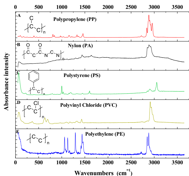
Fig. 3. Micro-Raman spectra of common virgin plastic polymers. A: Polypropylene (PP); B: nylon (PA); C: polystyrene (PS); D: polyvinyl chloride (PVC); E: polyethylene (PE).
