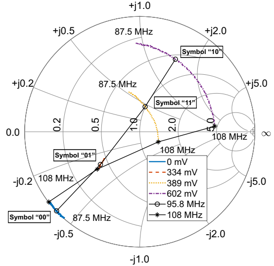
Fig. 4. Smith Chart with measured S_{11} values for 4 different voltage levels at the gate of transistor for P_{\text{in}} = -20 \text{ dBm} at 87.5 – 108 MHz.
