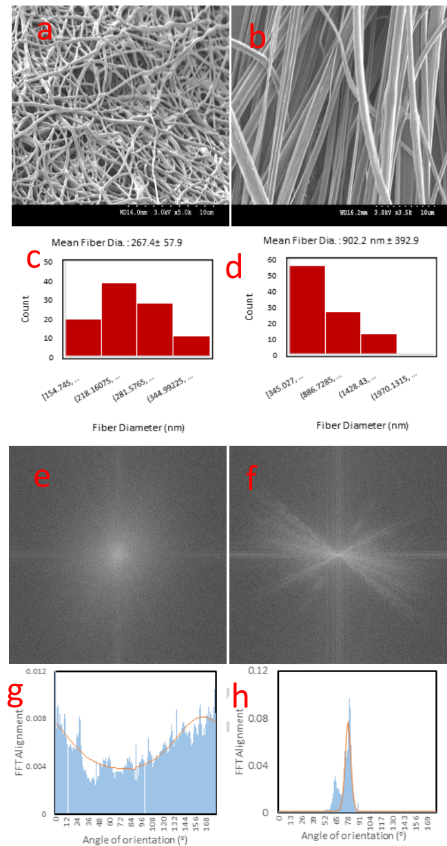
Figure 2 Investigation of morphology and alignment of the electrospun Nylon 66 nanofibers ( a, c, e, g) and ASC-g-P(MMA-co-EA) nanofibers (b, d, f, h). (a, b) SEM images of the Nylon 66 and ASC-g-P(MMA-co-EA) nanofibers collected by a rotating drum with constant rotary speed of 423 rpm, using a typical electrospinning setup and (c, d) fiber diameter frequency plots; (e, f) Image J Raw output of the 2-D FFT alignment analysis of electrospun fibers corresponding to SEM images in (a, b); (g, h) the directionality histogram reporting 2D-FFT alignment based on peak shape and the relative principle axis of orientation for the fibers.
