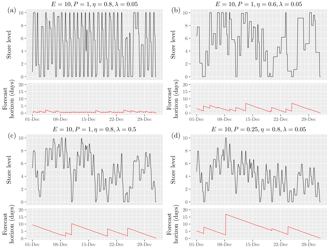
Figure 1: Examples in which the parameters associated with the store are varied. In each case, the upper plot shows the optimal level of storage and the lower plot shows the forecast horizon required at each stage of the optimisation.
