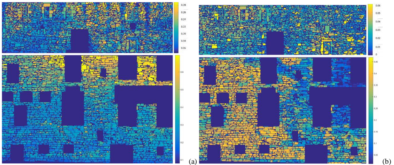
Figure 6. Stone maps for grayscale median values (a) and H_e coefficients (b).
