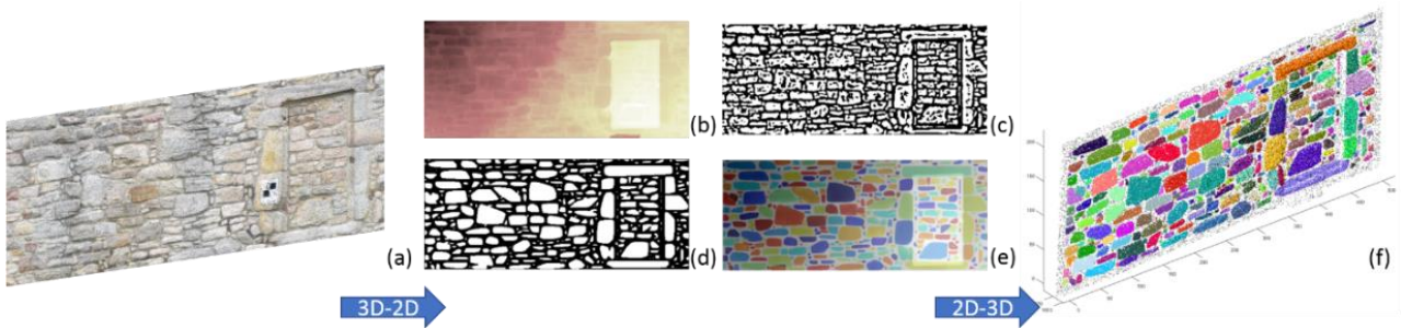
Figure 1. Summary of the rubble stone segmentation process. a) Input wall 3D point cloud, b) depth map, c) 2D CWT scalogram for the selected scale a, d) 2D stone segments after convex hull step, e) 2D stone segments after the final dilation step; and f) final segmentation re-mapped onto the 3D point cloud.
