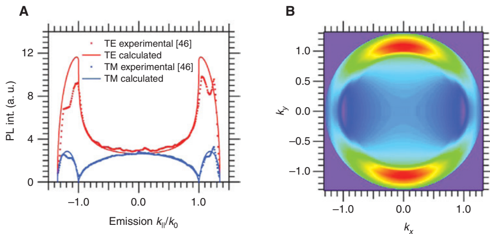
Figure 1: (A) Experimental (dotted lines) and calculated (solid lines) BFP cross-sections for the A exciton PL of SL MoS 2 . Experimental data have been obtained from Ref. [46]. (B) Polarized antenna-like radiation BFP image calculated from the TE and TM components shown in (A).
