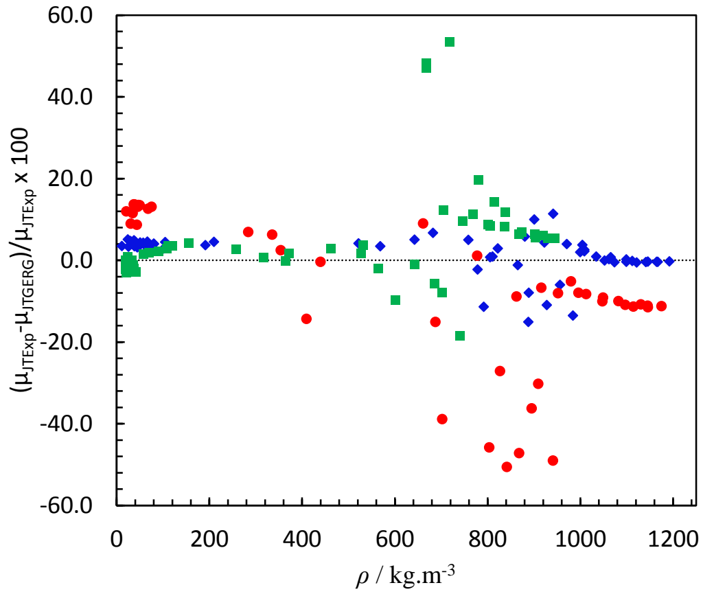
Figure 24. Deviation of Joule-Thomson Coefficient ( \mu_{\text{JT}} ) from GERG EoS for investigated mixtures, MIX 1: ( \blacklozenge ), MIX 2: ( \bullet ) and MIX 3: ( \blacksquare )
