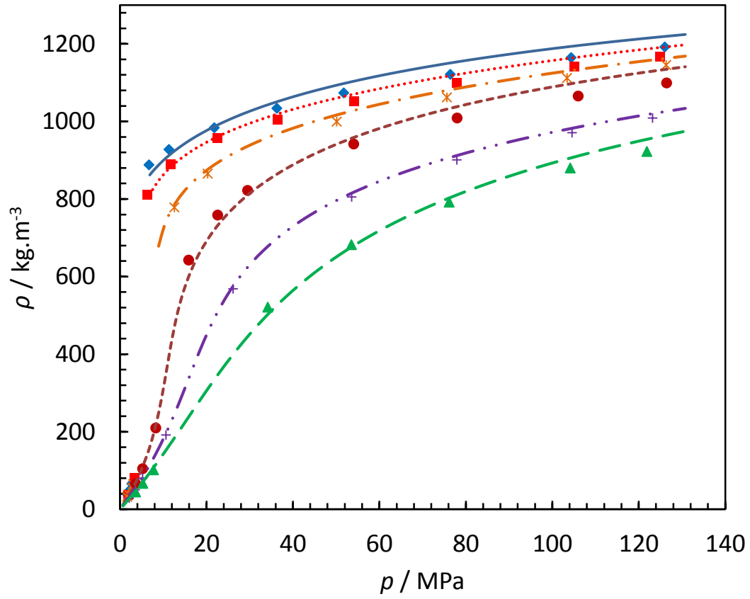
Figure 6. Experimental and modeling results of MIX 1 Experimental / modeling (PR-CO 2 ) results: (♦/—) at 273.15 K, (■/.....) at 283.15 K, (x/—.) at 298.15 K, (●/----) at 323.15 K, (+/—.) at 373.15 K and (▲/—) at 423.15 K
