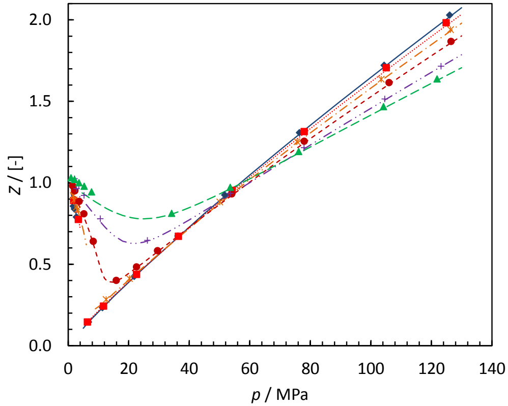
Figure 15. Compressibility factor for MIX 1 at different pressure ranges Experimental / modeling (GERG) results: ( \blacklozenge /—) at 273.15 K, ( \blacksquare /.....) at 283.15 K, ( \times /—) at 298.15 K, ( \bullet /- - -) at 323.15 K, ( + /—) at 373.15 K and ( \blacktriangle /—) at 423.15 K
