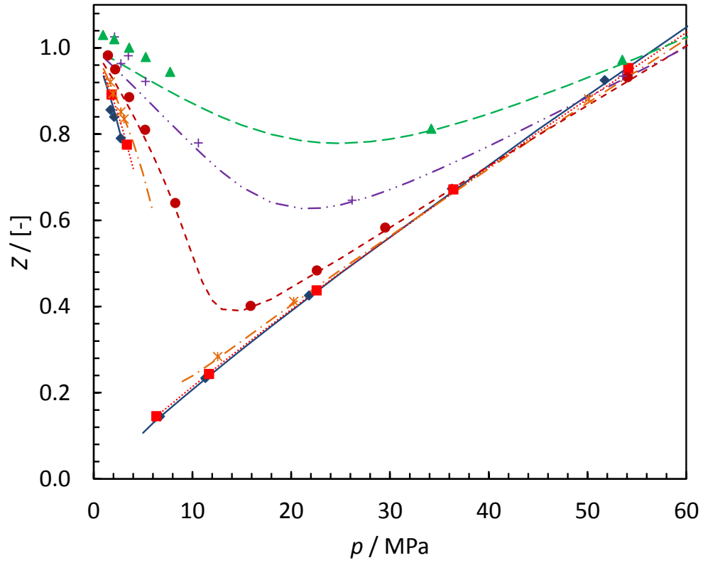
Figure 16. Compressibility factor for MIX 1 at lower pressure ranges Experimental / modeling (GERG) results: ( \diamond /—) at 273.15 K, ( \square /... ) at 283.15 K, ( \times /—) at 298.15 K, ( \bullet /- - -) at 323.15 K, ( + /—) at 373.15 K and ( \blacktriangle /—) at 423.15 K
