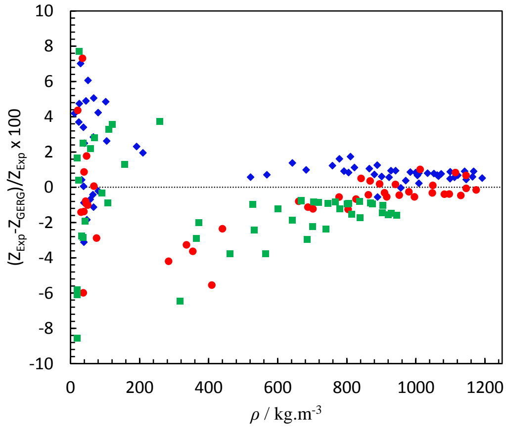
Figure 18. Deviation of compressibility factors ( Z ) from GERG EoS for investigated mixtures, MIX 1: ( \blacklozenge ), MIX 2: ( \bullet ) and MIX 3: ( \blacksquare )
