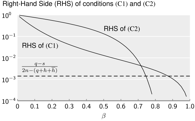
Figure 5. Values of the right-hand side (RHS) of conditions (C1) and (C2) from case 2) of Theorem 12, for the example of Fig. 1.
