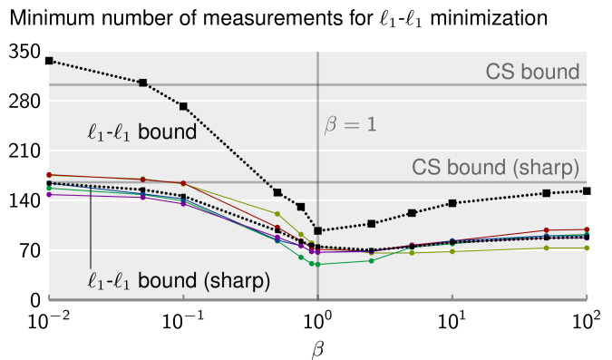
Figure 6. Experimental performance of \ell_1 - \ell_1 minimization for 5 different Gaussian matrices as a function of \beta (solid lines). The upper dotted line depicts the bounds of Theorem 12, which are minimized for \beta = 1 (vertical line). Horizontal lines: bound in (59) for CS and its sharp version in [60].
