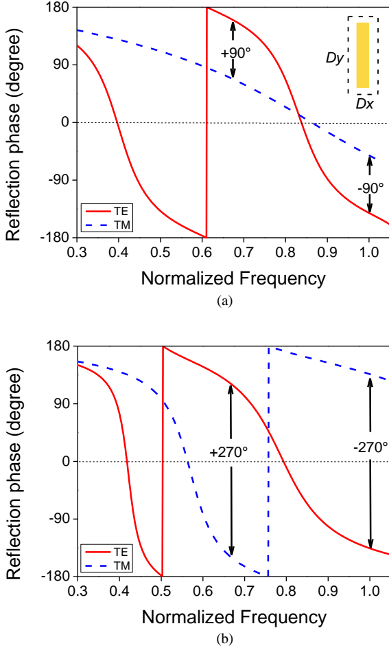
Fig. 3. Reflection phase sketches under normal LP incidence of (a) the design in [11] (inset: its unit cell) and (b) the proposed design.
