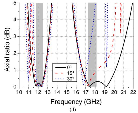
Fig. 6. Reflection coefficient and axial ratio under oblique incidence. (a, c) Incident angle varies in xz -plane. (b, d) Incident angle varies in yz -plane.
