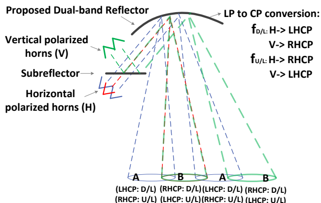
Fig. 1. Illustration of problem for contiguous multibeam coverage in Single Feed per Beam configuration; for contiguous beams ‘A’ and ‘B’, the blue and red feeds physically overlap. The proposed scheme exploits a linear polarization (e.g. wire grid) selective subreflector and a dual-band orthogonal linear to circular main reflector to enable the feeds associated with beams ‘B’ to be at a physically different location.
