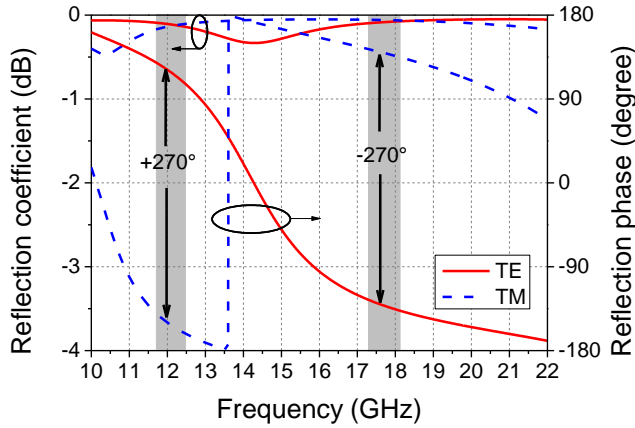
Fig. 5. Reflection coefficient and phase response under normal incidence.
