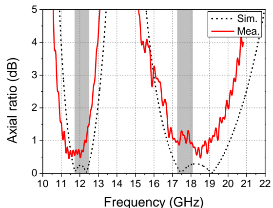
Fig. 8. Comparison of measured and simulated axial ratio performance under an incident angle of 2^\circ in xz -plane. (noted that bistatic horns configuration was utilized in the measurement)
