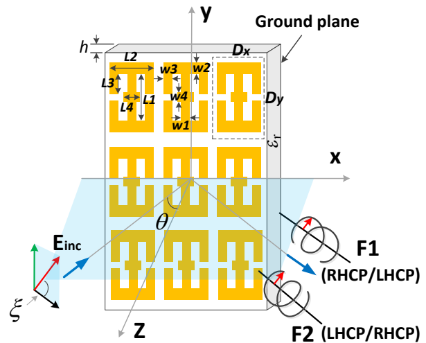
Fig. 2. Geometrical configuration and operation principle.
