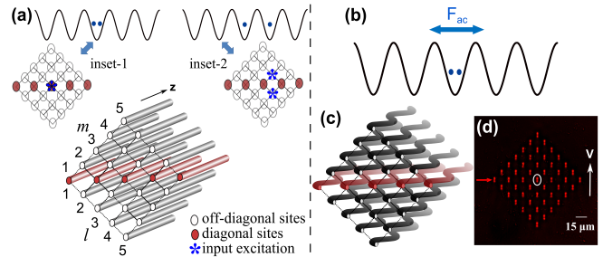
FIG. 1: (a) Schematic diagram of a photonic square lattice where the diagonal sites l=m (shown in red) have a shifted propagation constant, \Delta\beta \equiv [U_0, \text{the on-site interaction energy}] compared to the off-diagonal waveguides. The excitation of a diagonal waveguide at the input is the optical analog of two interacting particles at the same potential well of a one-dimensional lattice at time t = 0 (inset-1). The excitation of the two off-diagonal waveguides corresponds to the particles located at different lattice sites at t = 0 (inset-2); see also Ref. [30]. (b) Schematic diagram of two interacting particles in a one-dimensional lattice driven by a sinusoidal force ( F_{ac} ). (c) A modulated photonic square lattice which mimics the dynamics of (b). (d) Micrograph of the facet of a laser-fabricated photonic square lattice. The lattice axes were rotated by 45^\circ with respect to the vertical direction (V) to achieve \kappa_x \approx \kappa_y = \kappa (see APPENDIX). The circled waveguide was excited at the input for all measurements. The red arrow indicates the main diagonal ( l = m ).
