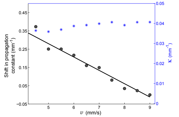
FIG. A1: Experimentally measured variation of shift in propagation constant [\beta(v) - \beta(v = 9 \text{ mm/s})] as a function of translation speed, v (filled circles). The solid line is the linear fit. (Blue stars) The variation of hopping amplitude ( \kappa ) with translation speed can be ignored as it is comparable to the random variation of \kappa (i.e. the off-diagonal disorder).
