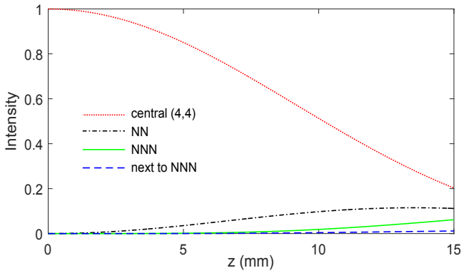
FIG. A2: Variation of light intensity along the propagation direction, z , for a photonic square lattice. Here \Delta\beta=0 , A=0 and \kappa=0.04 \text{ mm}^{-1} . The red curve is for the central waveguide that was excited at the input ( z=0 ). The black, green and the blue curves indicate intensities at the nearest neighbor (NN), next-nearest neighbor (NNN) and next to next-nearest neighbor waveguides. Fig. 2 (a) shows the measured output intensity distribution at z=15 \text{ mm} .
