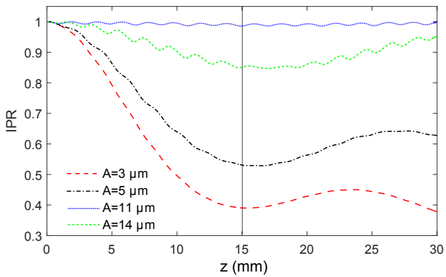
FIG. A3: Variation of inverse participation ratio (IPR) as a function of propagation distance, z , for the modulated photonic lattices presented in Fig. 4 (a)-(d). The solid black line indicates the z value where the output intensities were experimentally measured.
