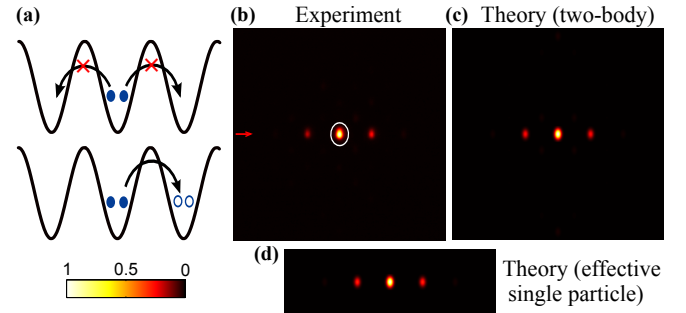
FIG. 3: (a) Schematic diagram of pair hopping in the strong-interaction regime [ U_0 \gg J ]. (b) Experimental observation of pair hopping in the 70-mm-long straight photonic square lattices for \kappa = 0.027 \text{ mm}^{-1} , \Delta\beta = -0.21 \text{ mm}^{-1} . The corresponding two-body simulation and the effective single-particle simulation with pair coupling \kappa_2 = -2\kappa^2/\Delta\beta , are shown in (c) and (d), respectively. Each image is normalized such that the total output power is 1. The white circle indicates the waveguide that was excited at the input.
