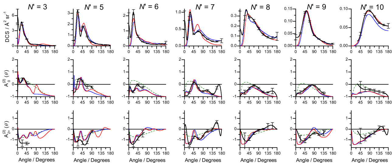
FIG. 4. Differential cross sections and rotational angular momentum polarization moments, A_{q+}^{(2)}(\theta) , for the inelastic collisions of NO(A) with Ne at \langle E_{col} \rangle = 523 \text{ cm}^{-1} for product states N' = 3 and 5-10. Black line: results of fitting to experimental images (error bars represent 95% confidence limits), red line: results of energy averaged QS calculations run on the CF PES, blue line: results of energy averaged QS calculations run on the PRRH PES, dashed green (for A_{q+}^{(2)}(\theta) only): results of energy averaged kinematic apse calculations.
