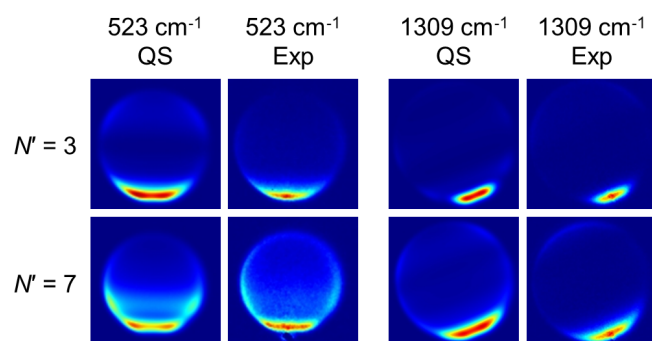
FIG. 8. Comparison of simulated V + H images, using the results of QS calculations on the CF PES, to experimental V + H images for N' = 3 and 7, at \langle E_{col} \rangle = 523 cm -1 and \langle E_{col} \rangle = 1309 cm -1 .
