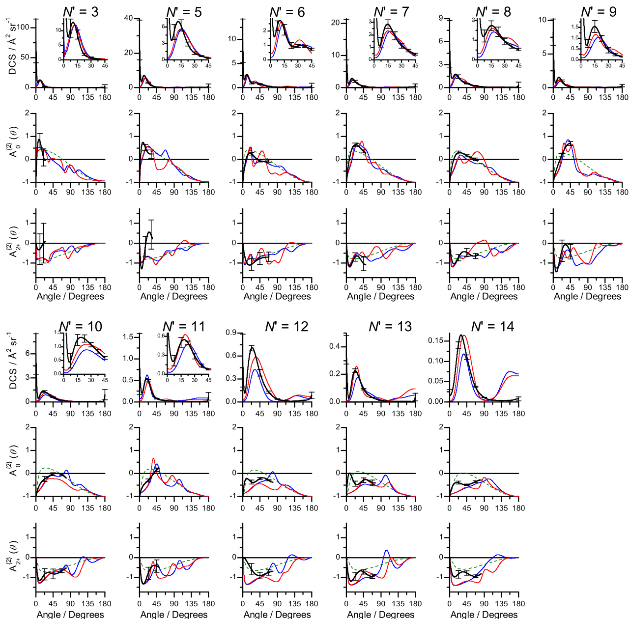
FIG. 5. Differential cross sections and rotational angular momentum polarization moments, A_{q+}^{(2)}(\theta) , for the inelastic collisions of NO(A) with Ne at \langle E_{col} \rangle = 1309 \text{ cm}^{-1} for product states N' = 3 and 5-14. Black line: results of fitting to experimental images (error bars represent 95% confidence limits), red line: results of energy averaged QS calculations run on the CF PES, blue line: results of energy averaged QS calculations run on the PRRH PES, dashed green (for A_{q+}^{(2)}(\theta) only): results of energy averaged kinematic apse calculations.
