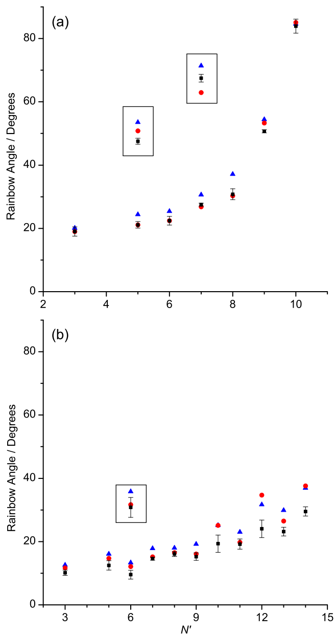
FIG. 7. Plots showing the rotational rainbow angle of the DCSs, as a function of N' at (a) \langle E_{col} \rangle = 523 \text{ cm}^{-1} , (b) \langle E_{col} \rangle = 1309 \text{ cm}^{-1} . Black squares, experimental results; red circles, QS calculation results from the CF PES; blue triangles, QS calculation results from the PRRH PES. Points enclosed by boxes are the maxima for the second rainbow feature apparent in the DCS for states where these features are clearly distinguishable. Experimental points are the mean from multiple independent measurements of the DCS, error bars represent 2 standard errors of the mean.
