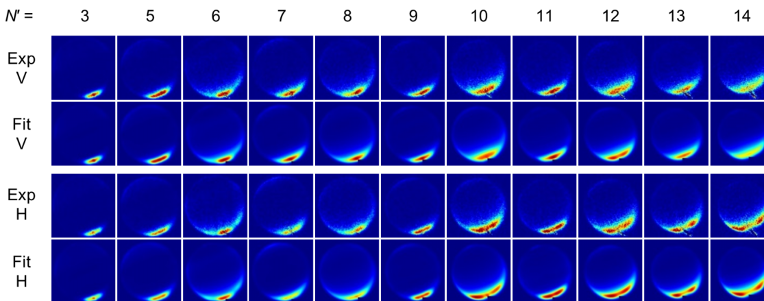
FIG. 3. Single acquisition experimental images for the inelastic collision of NO(A, v=0, N=0, j=0.5 ) with Ne at \langle E_{col} \rangle = 1309 \text{ cm}^{-1} , for product states N' = 3 and 5-14, and for both H and V probe laser polarizations, together with images obtained from the fitting routine.
