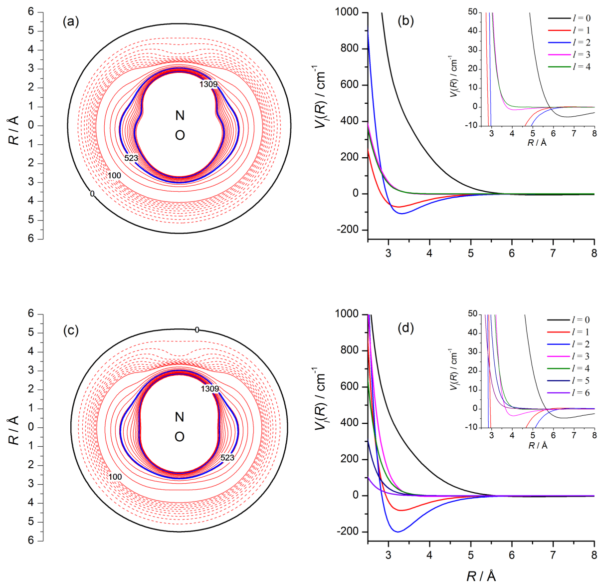
FIG. 6. ((a) and (c)) Polar contour plots of the PRRH and CF PES, respectively. Solid black contour, 0 \text{ cm}^{-1} . Dashed red contours, 0-100 \text{ cm}^{-1} in 10 \text{ cm}^{-1} intervals. Solid red contours, 100-1500 \text{ cm}^{-1} in 100 \text{ cm}^{-1} intervals. Solid blue contours, 523 \text{ cm}^{-1} and 1309 \text{ cm}^{-1} , representing the two average collision energies used in the experiments. ((b) and (d)) Radial dependence of the Legendre moments of the PRRH and CF PES, respectively, with insets on an expanding vertical scale to show the shallow, long-range isotropic wells present on both surfaces.
