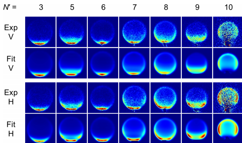
FIG. 2. Example single acquisition experimental images for the collision of NO(A, v = 0, N = 0, j = 0.5 ) with Ne at \langle E_{col} \rangle = 523 \text{ cm}^{-1} , for product states N' = 3 and 5-10, and for both H and V probe laser polarizations, together with images obtained from the fitting routine.
