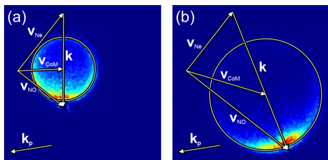
FIG. 1. Newton diagrams for the collision of NO(A) with Ne at (a) \langle E_{col} \rangle = 523 \text{ cm}^{-1} and (b) \langle E_{col} \rangle = 1309 \text{ cm}^{-1} overlaid on V + H experimental images for the product state N' = 8 . Arrows indicate the velocity vectors of the colliders: \mathbf{v}_{NO} , \mathbf{v}_{Ne} , the center of mass velocity: \mathbf{v}_{CoM} , and the relative velocity vector: \mathbf{k} . The ring represents the mean velocity of NO scattered into the plane of the detector. \mathbf{k}_p indicates the propagation direction of the probe laser beam.
