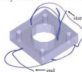
Fig. 4, Probe motion chronocyclegraph
